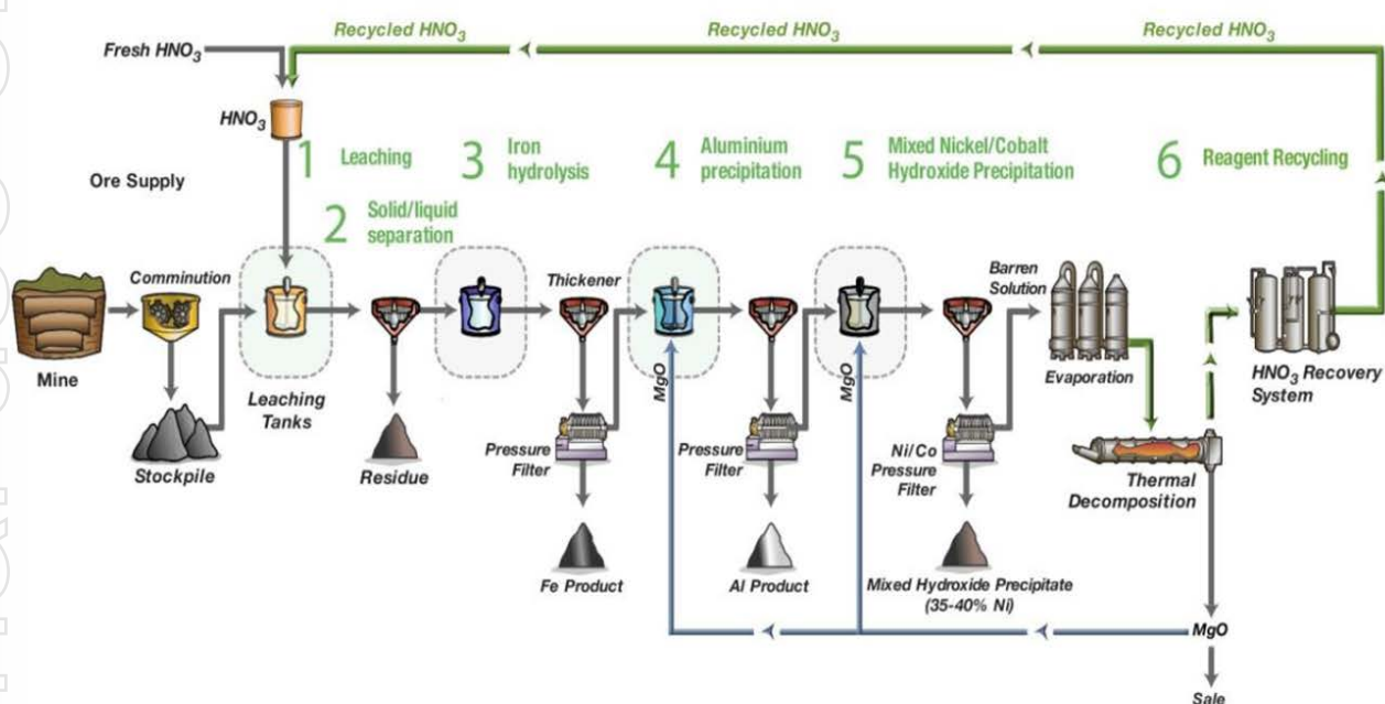
Fig 1. Simplified Schematic of the DNI Process™
