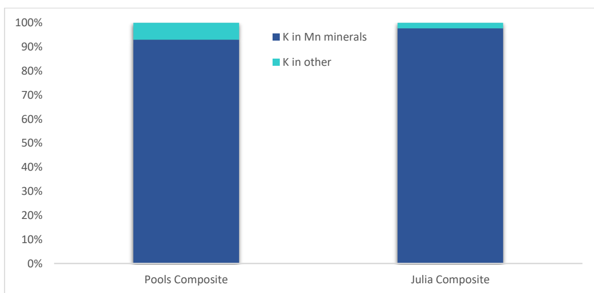
Figure 2: QEMSCAN potassium deportment analysis. The majority of potassium reports to manganese minerals.
