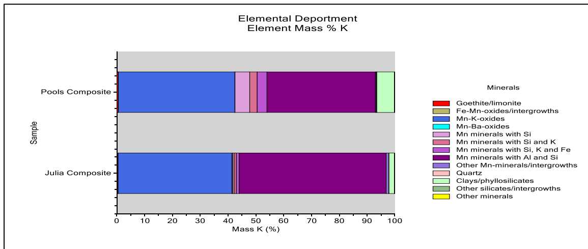
Figure A-2: QEMSCAN elemental deportment to potassium showing the relatively high content of Mn (manganese) associated with K (potassium) that could improve leach kinetics (Source: METS Engineering).
