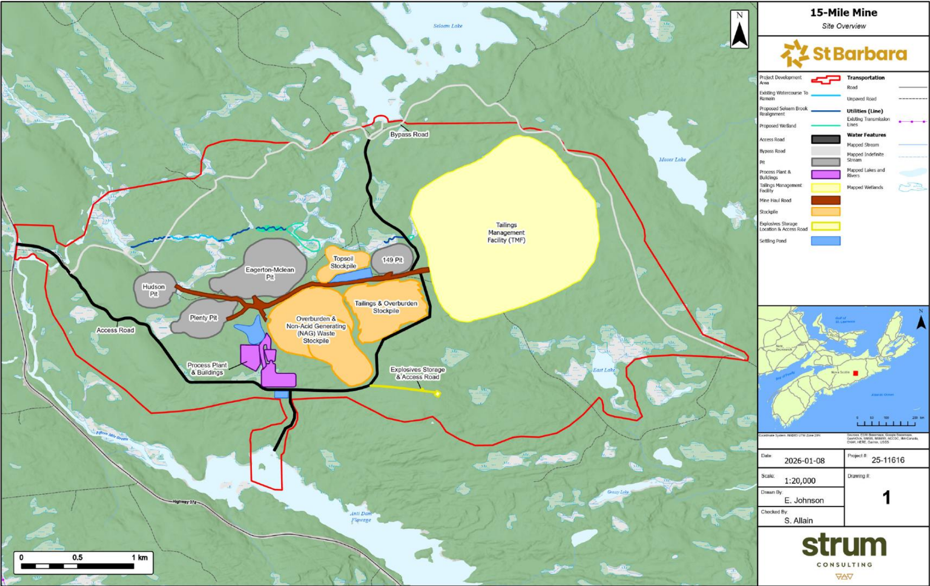
Figure 2: 15-Mile Processing Hub Layout
