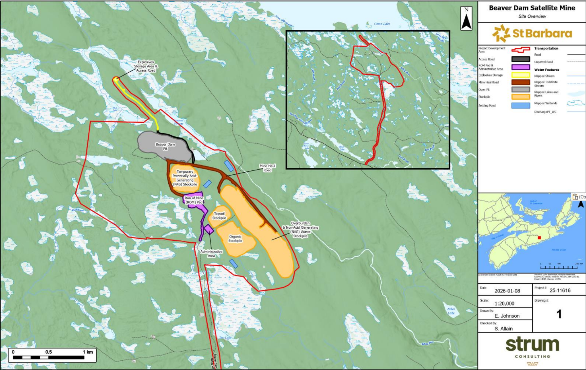
Figure 4: Beaver Dam Satellite Mine Layout
