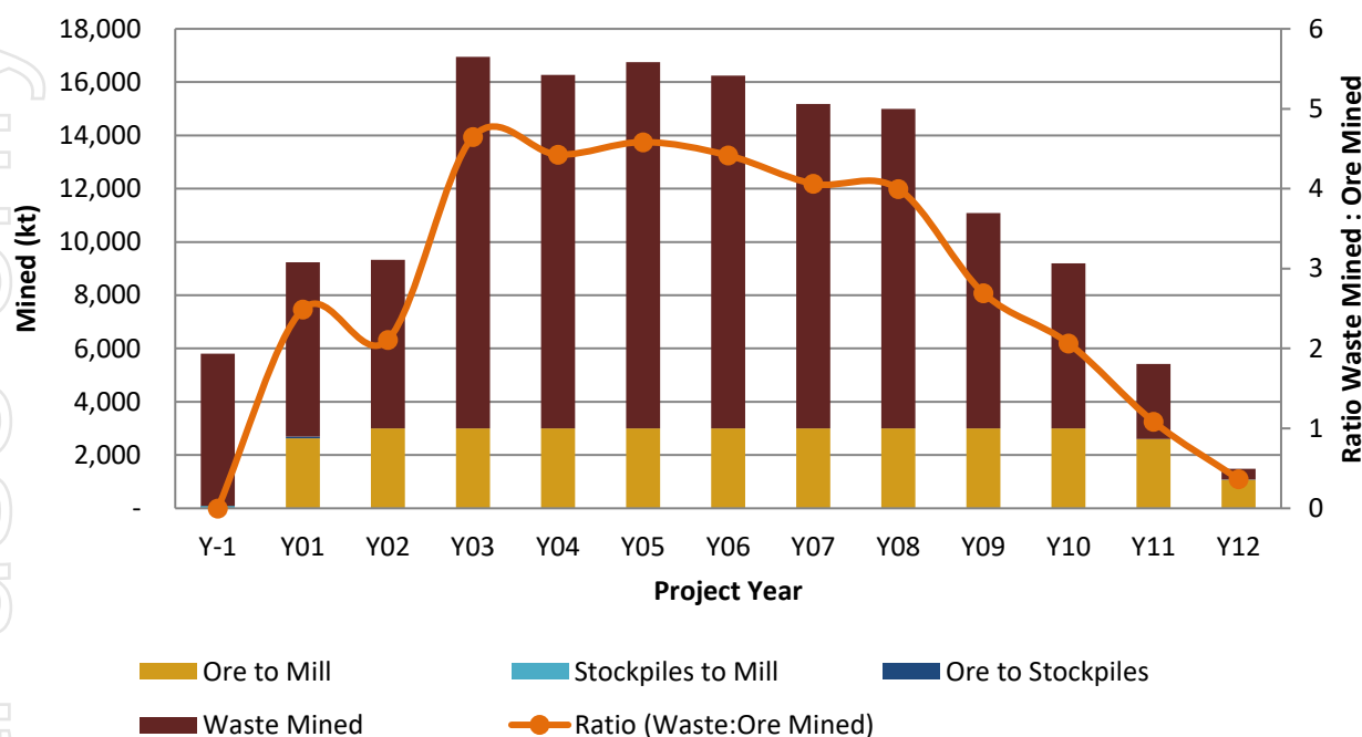
Figure 9: Mine Plan Production Summary
