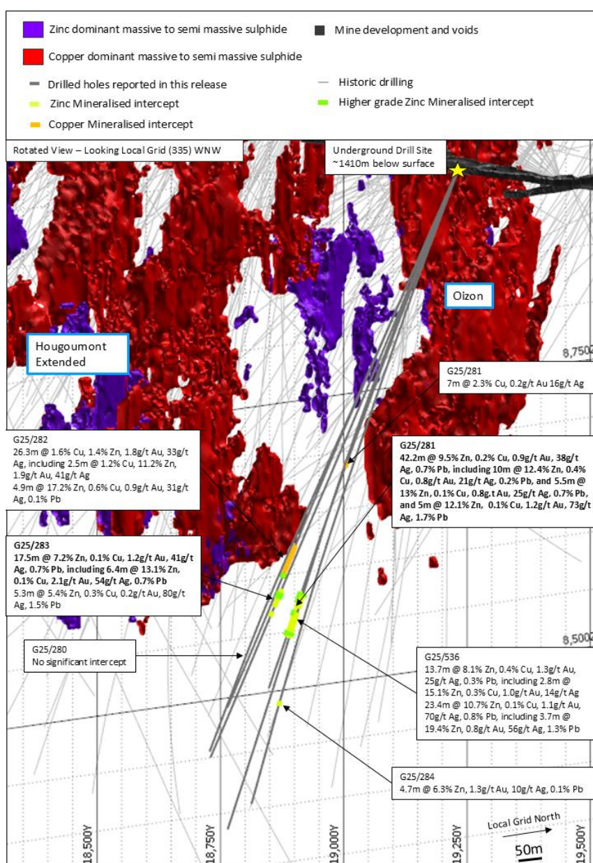
Figure 4 – Rotated-section view looking local grid west-north-west displaying Oizon and Hougoumont Extended, sulphide lenses, and mining voids. Highlighted drill hole traces reported in this release and historic drilling.
