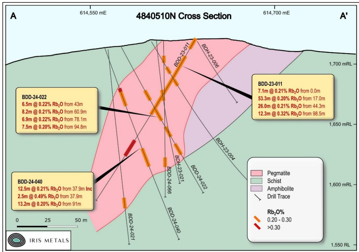
Figure 2: Section A-A'
