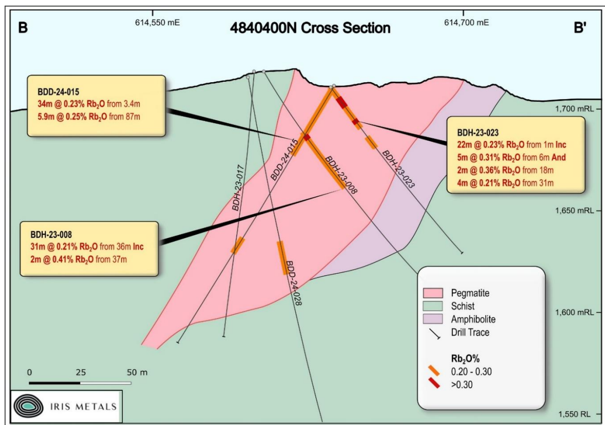
Figure 3: Section B-B'
