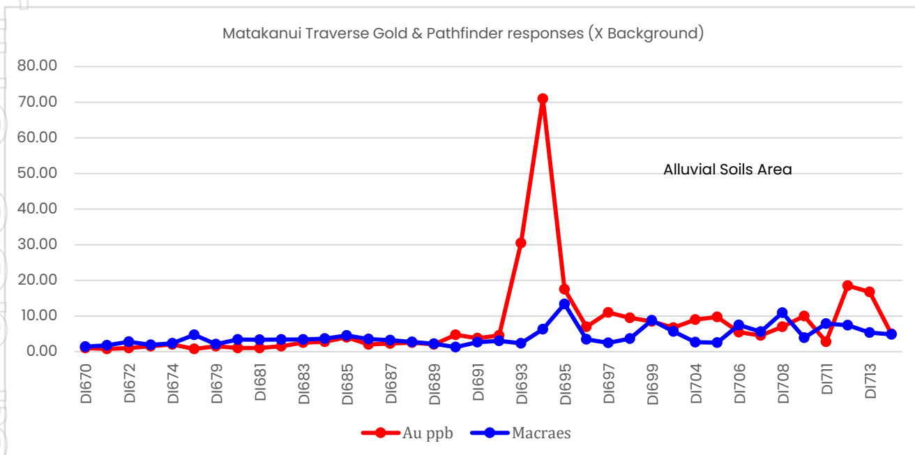
Figure 4: Gold and Pathfinder responses along Matakanui traverse
