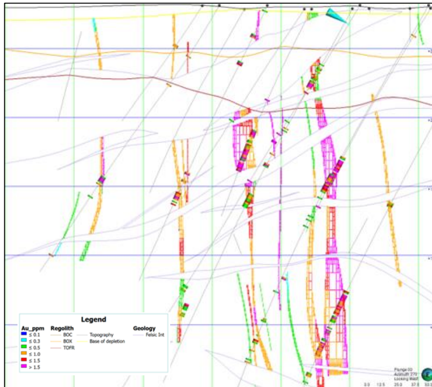
Figure 11: Fiama deposit cross-section 424,100mE \pm 25m, looking MGA Zone 51 Bearing 270°, showing estimated gold grades in the Mineral Resource block model and drill holes showing gold grades. The grid squares represent 50m.
