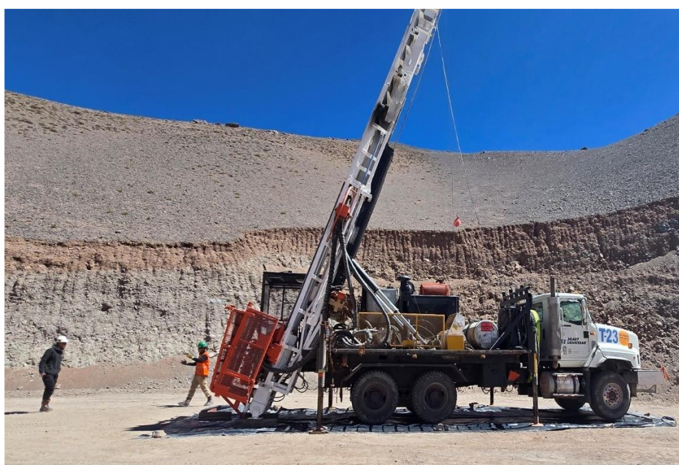
Figure 1: Boart Longyear's diamond drill LF230 lining up on pad TMT-TC-DDH-001.
