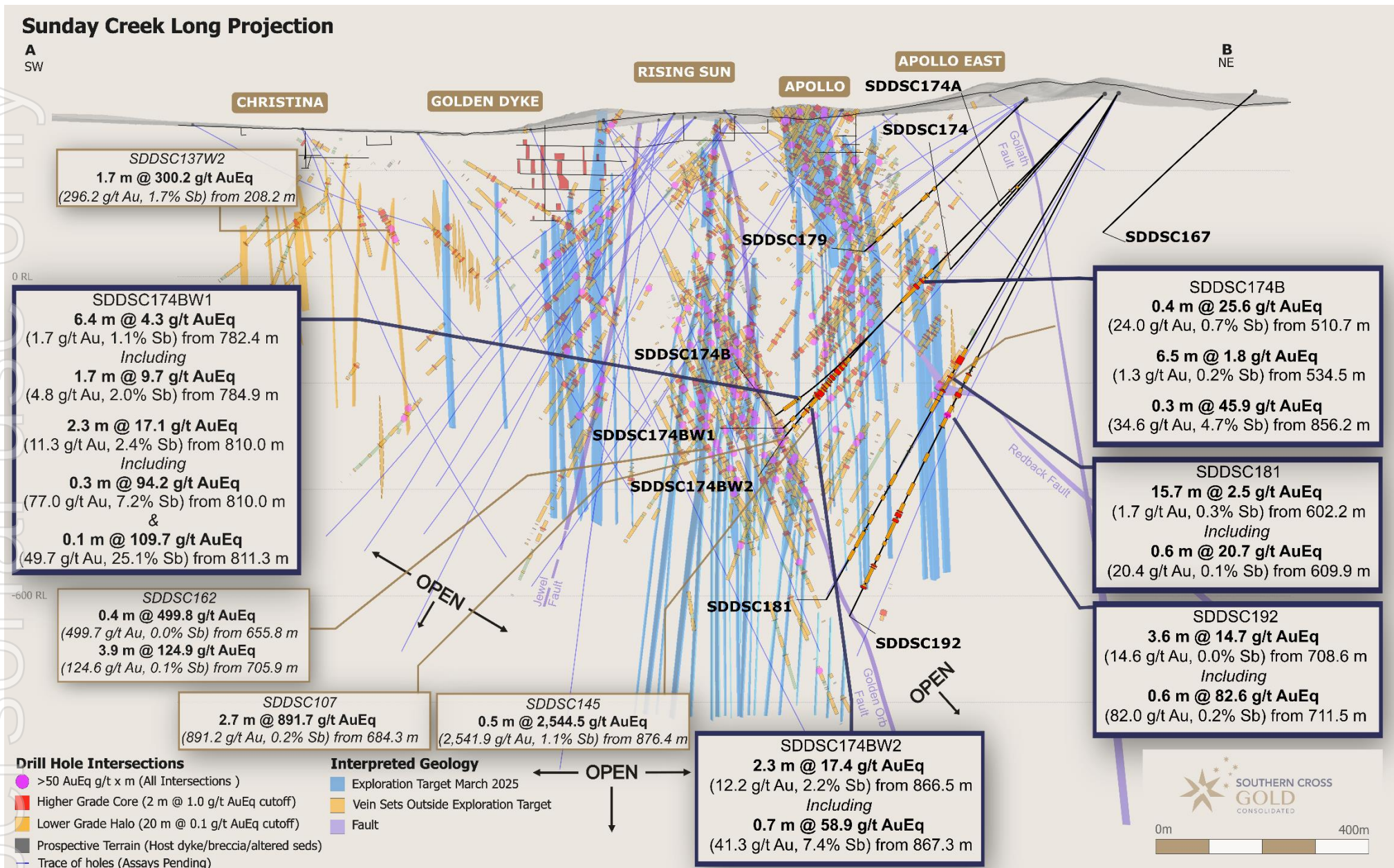
Figure 3: Sunday Creek longitudinal section across A-B in the plane of the dyke breccia/alterd sediment host looking towards the north (striking 236 degrees) showing mineralized vein sets. Showing holes SDDSC167, SDDSC174, SDDSC174A, SDDSC174B, SDDSC174BW1, SDDSC174BW2, SDDSC179, SDDSC181, SDDSC183, SDDSC185, SDDSC189 and SDDSC192 reported here (dark blue highlighted box, black trace), with selected intersections and prior reported drill holes. The vertical extents of the vein sets are limited by proximity to drill hole pierce points.
