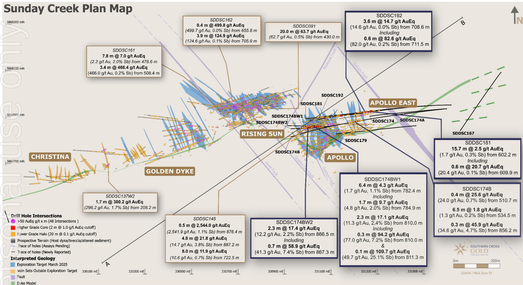
Figure 1: Sunday Creek plan view showing selected results from holes SDDSC167, SDDSC174, SDDSC174A, SDDSC174B, SDDSC174BW1, SDDSC174BW2, SDDSC179, SDDSC181, SDDSC183, SDDSC185, SDDSC189 and SDDSC192 reported here (dark blue highlighted box, black trace), with selected prior reported drill holes.
