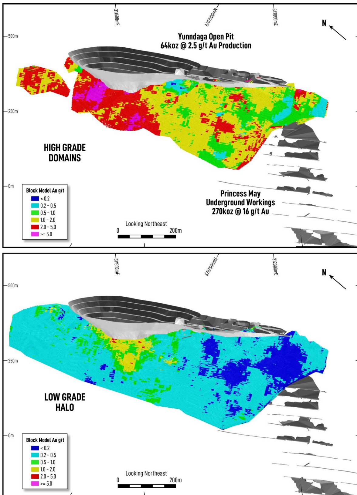
Figure 3: 3D Schematics of the Yunnadaga Resource Model coloured by Grade. High Grade domains are contained within a lower grade envelope illustrated above.
