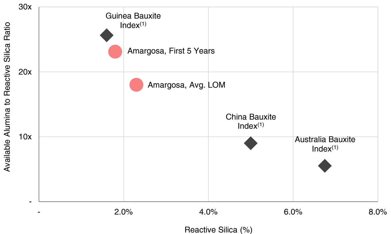
Amargosa Product Quality vs. Key Bauxite Indices
