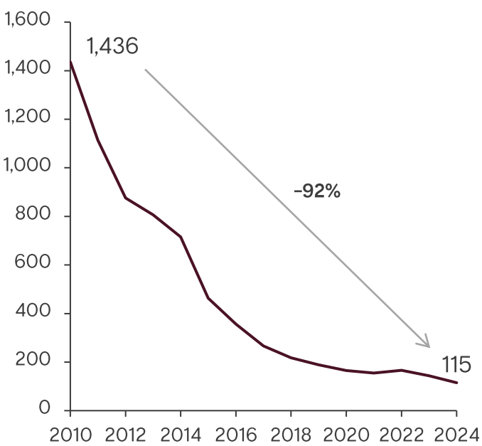
Li-ion battery price Real 2024 $/kWh
