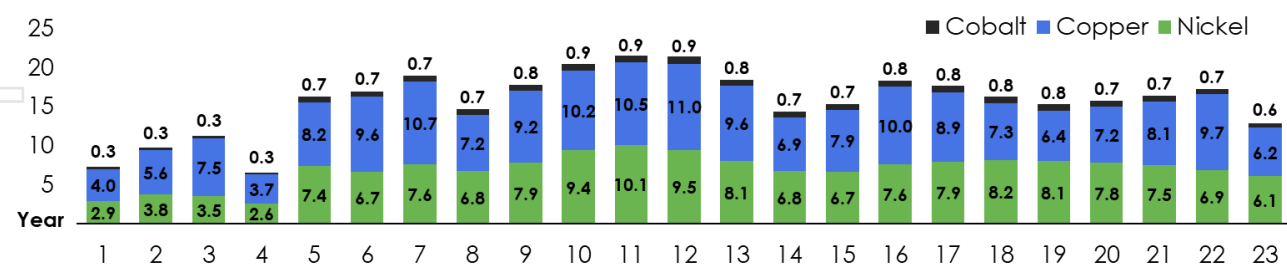
Figure 22. Gonneville base metal production profile (recovered).
