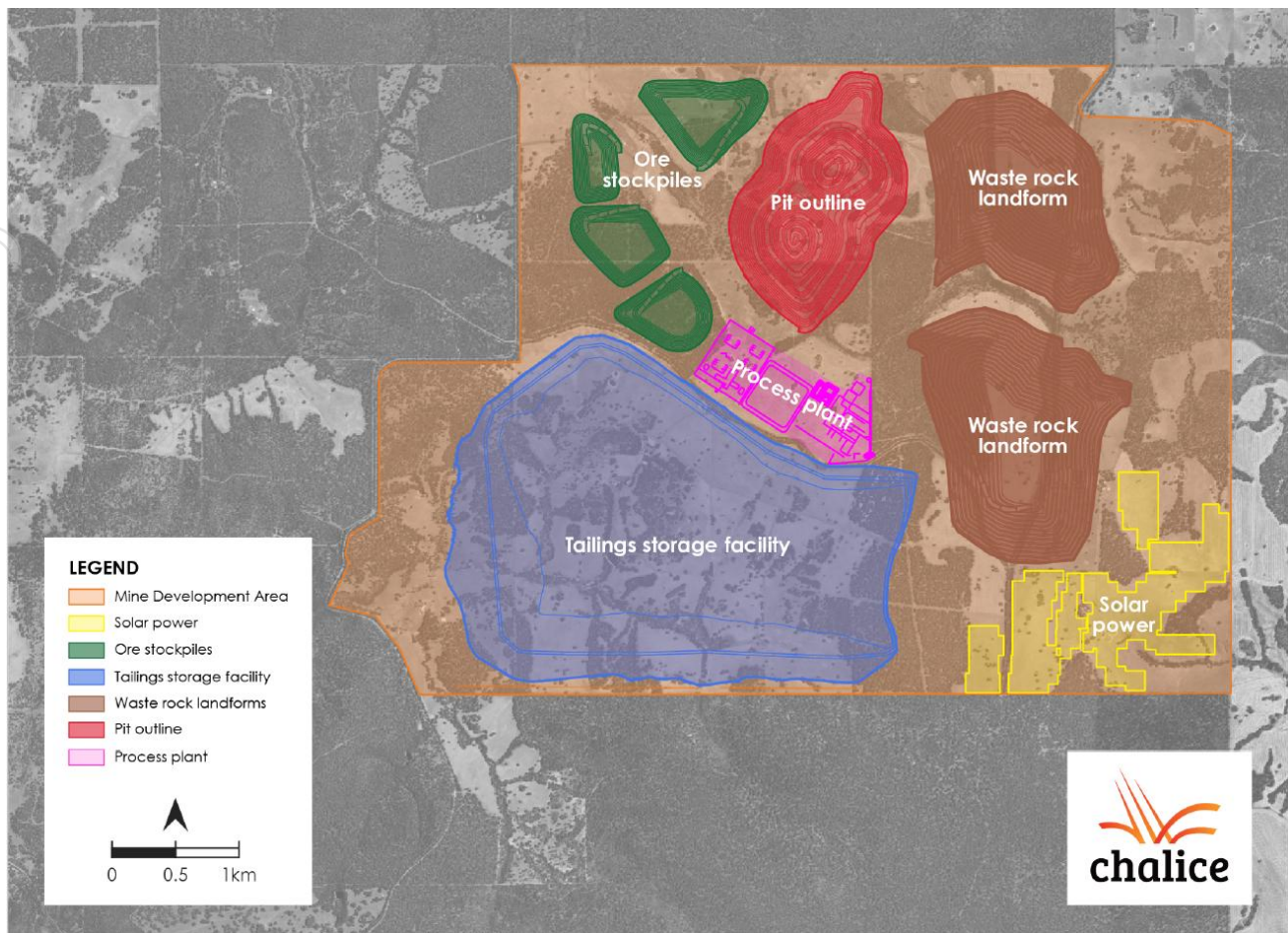
Figure 12. Gonneville MDA preliminary site layout.
