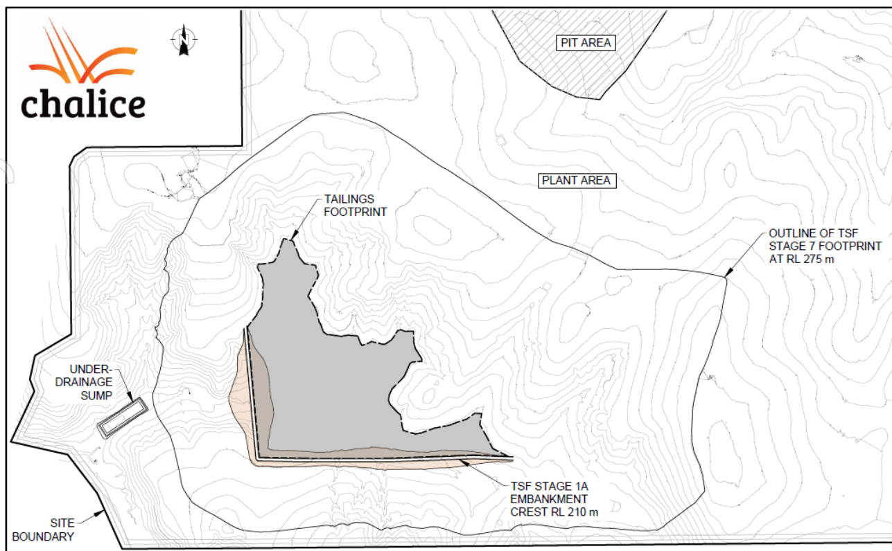
Figure 30. TSF Plan Lift 1A (Year 3).
