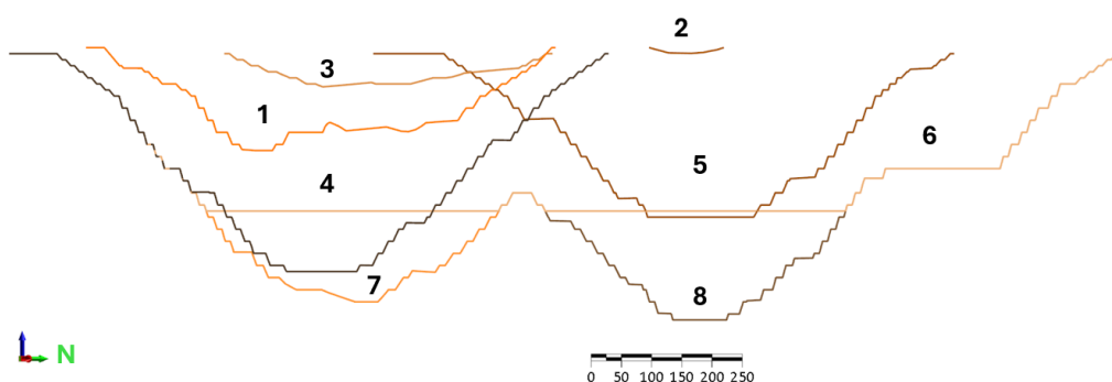
Figure 12. NS section view (looking west) of the modelled open-pit phases.
