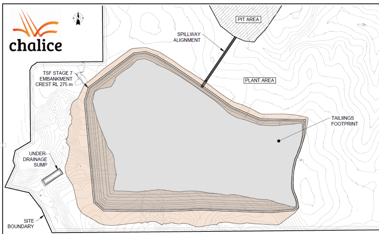
Figure 31. TSF Plan Lift 7 (final design lift).
