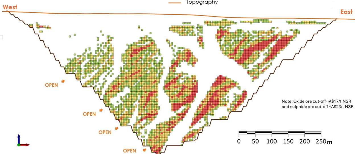
Figure 18. EW Section view 2 (looking North) of ore blocks by NSR within the modelled pit.
