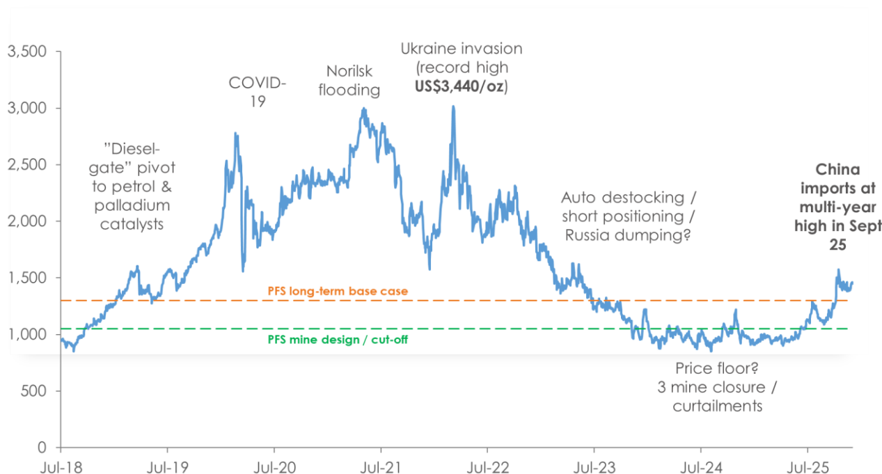
Figure 9. LBMA palladium price (blue), PFS mine design and PFS long term price, US$/oz.
