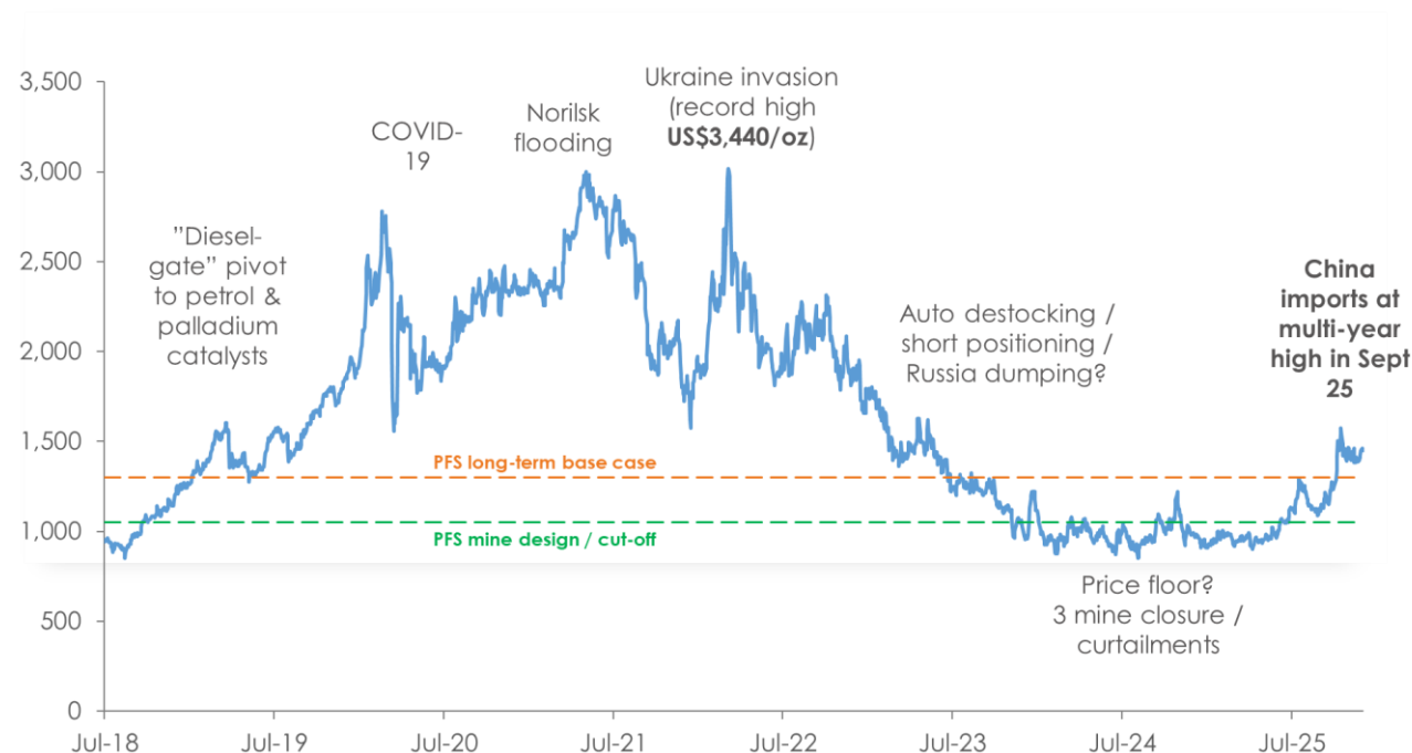
Figure 44. LBMA palladium price (blue), PFS mine design and PFS long term price, US$/oz.
