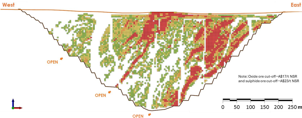
Figure 17. EW Section view 1 (looking North) of ore blocks by NSR within the modelled pit.
