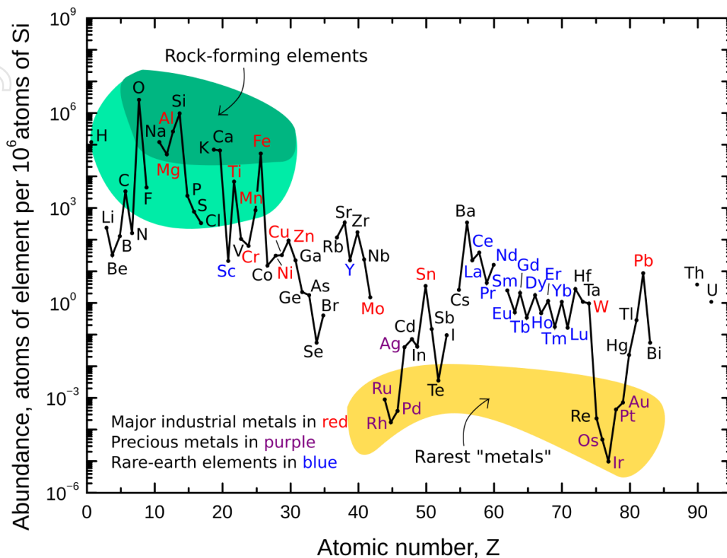
Figure 2. Abundance (atom fraction) of the chemical elements in Earth's upper continental crust as a function of atomic number.
