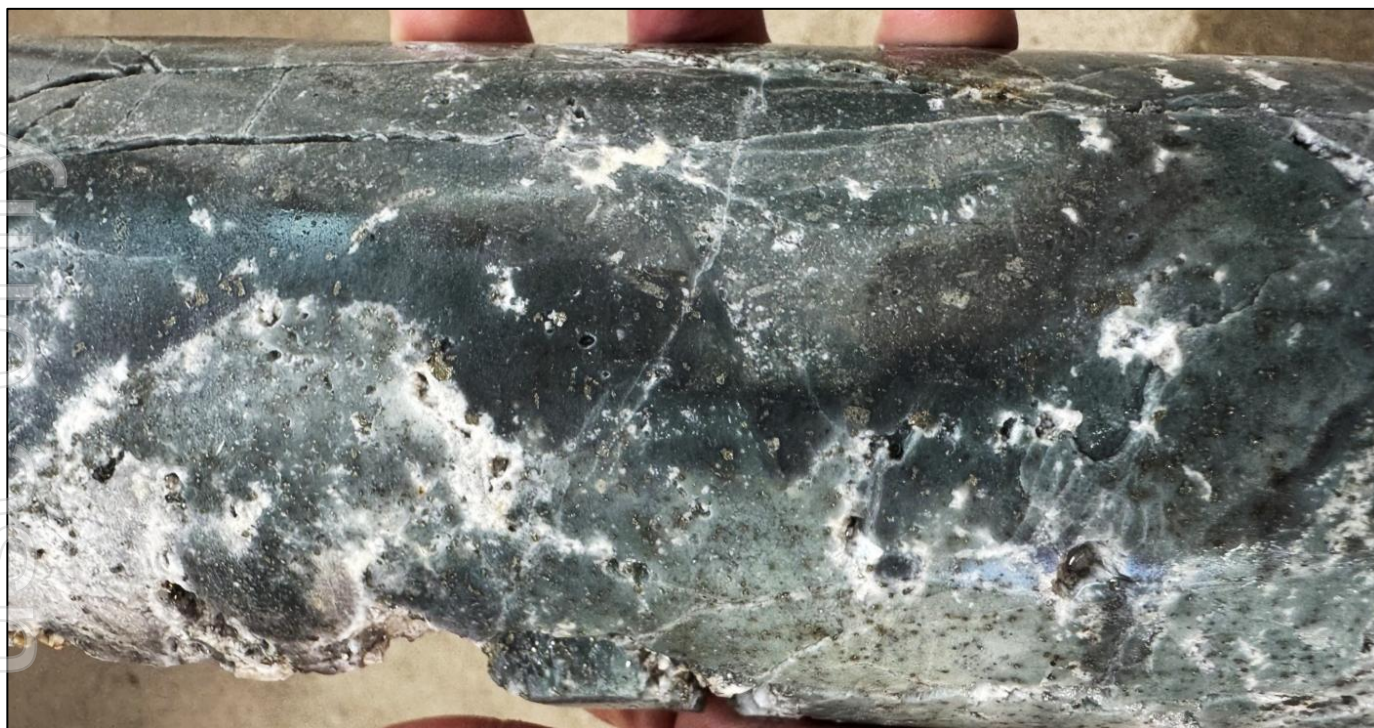
Figure 4. Core photograph of ZRSD25200A from 318.1m to 320.1 m of chloritized quartz-diorite with disseminated pyrite and carbonate cavities –6.0g/t Au.
