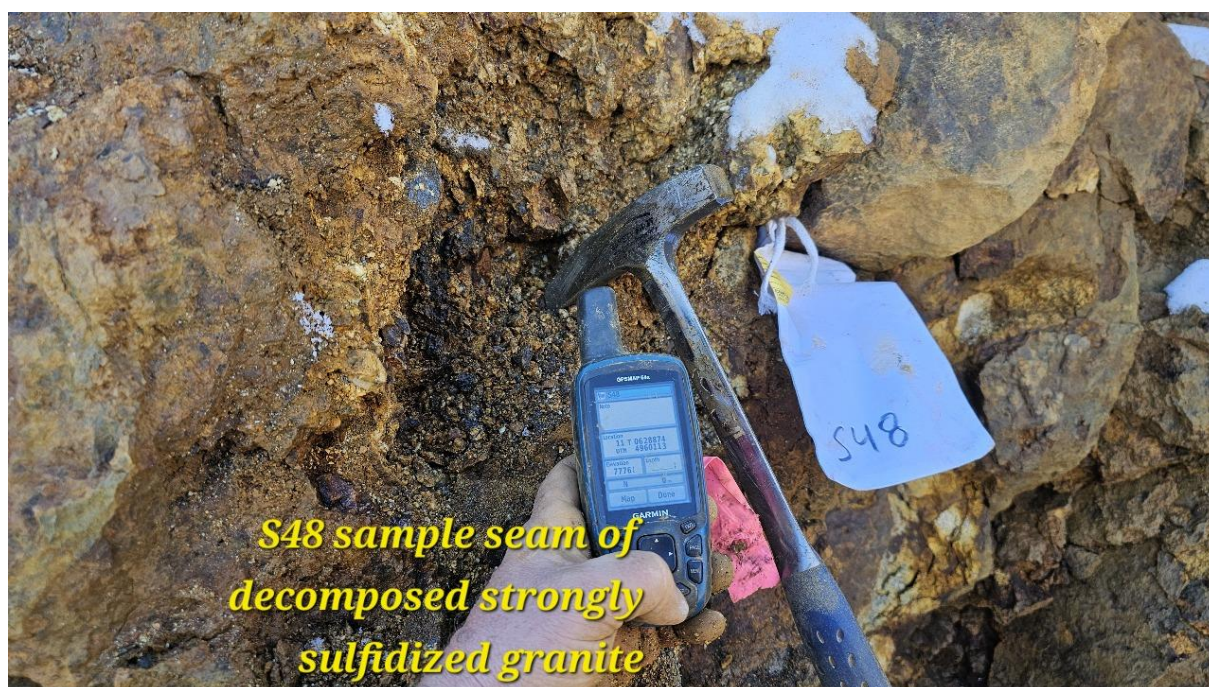
Figure 5: Photo showing sample S48 at Springfield Prospect, here we see strongly oxidised sulphides in granite which returned 7.75 g/t Au and 0.1% WO 3 (see table 1 and appendix B)
