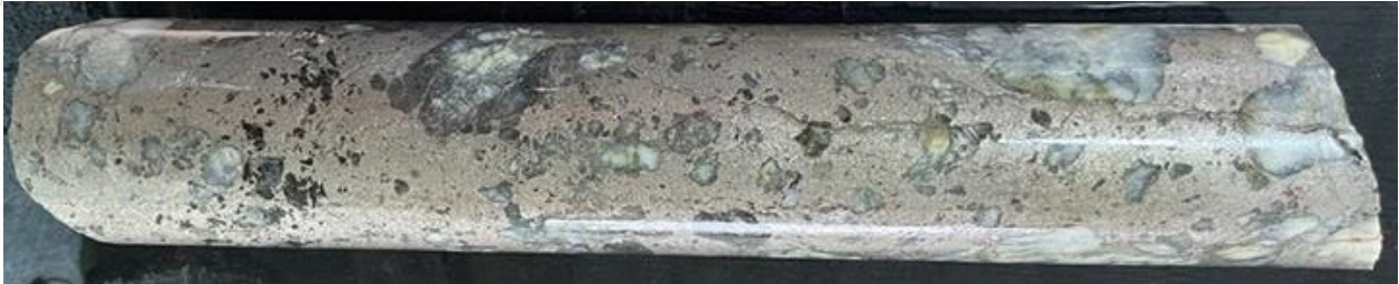
Figure 4. Core photo – massive sulphide breccia from ATDD001 at approximately 413m downhole. Dominantly pyrrhotite with minor chalcopyrite replacing quartz-carbonate. Core diameter is 50.5mm.
