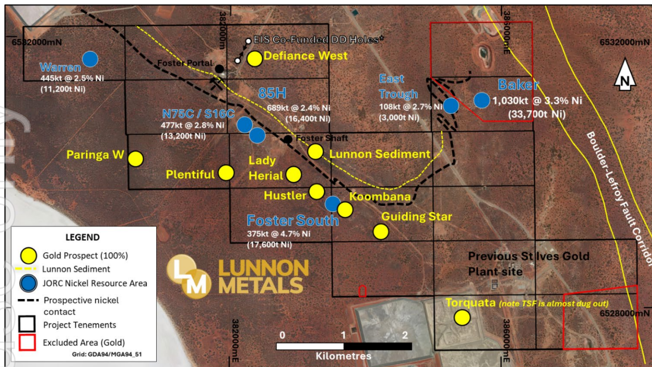
Figure 3: Foster-Baker Project Area showing select high-ranking gold prospects, & nickel Mineral Resource 7 positions.
