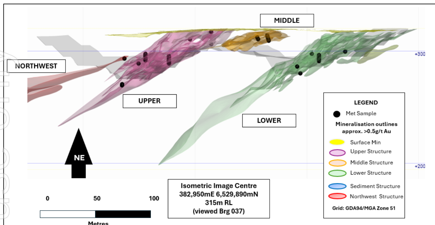
Figure 15: Long section view (150m wide) of the Lady Herial system showing location of metallurgical samples.
