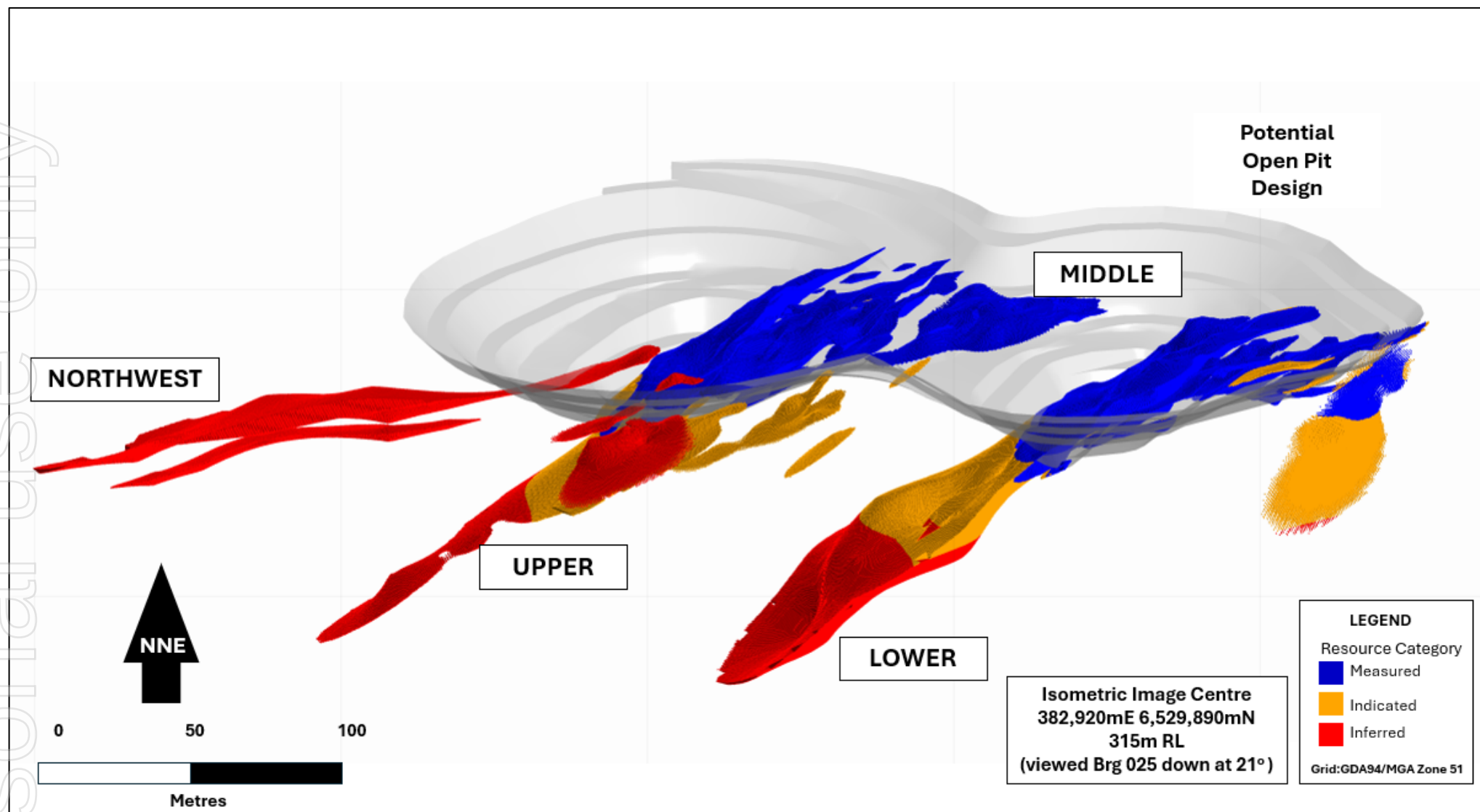
Figure 14: Isometric view, looking down and toward the NNE, of the Lady Herial gold deposit illustrating the Upper, Lower, Middle and Northwest Structures coloured by Mineral Resource classification categories.
