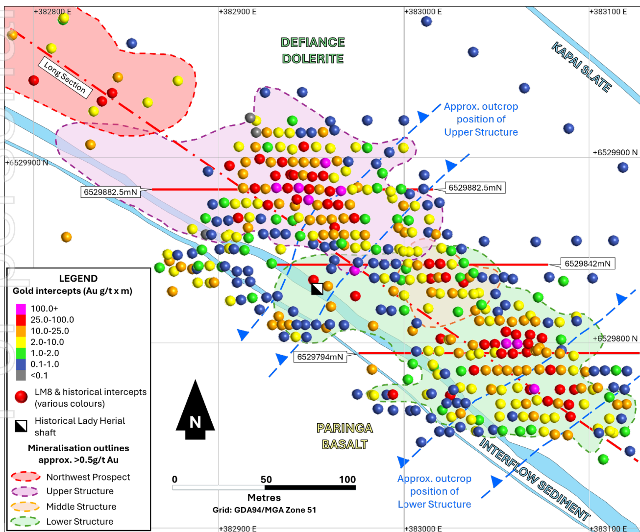
Figure 4: Plan view at the Lady Herial deposit scale, illustrating all drilling along with location of long section shown in Figure 5 and cross sections in Figures 6, 7 and 8.
