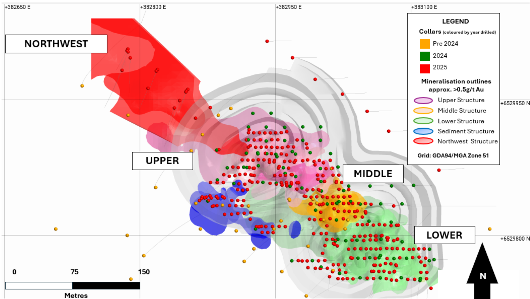
Figure 10: Plan View of the Lady Herial gold deposit illustrating all drilling coded by period drilled and a potential open pit design.
