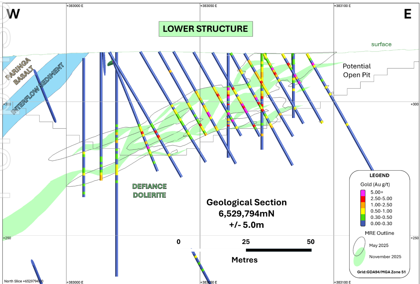
Figure 8: Geological cross section through the Lower Structure showing the current more discrete modelled high grade lenses against the 7 May 2025 MRE outline (with a potential open pit shell).
