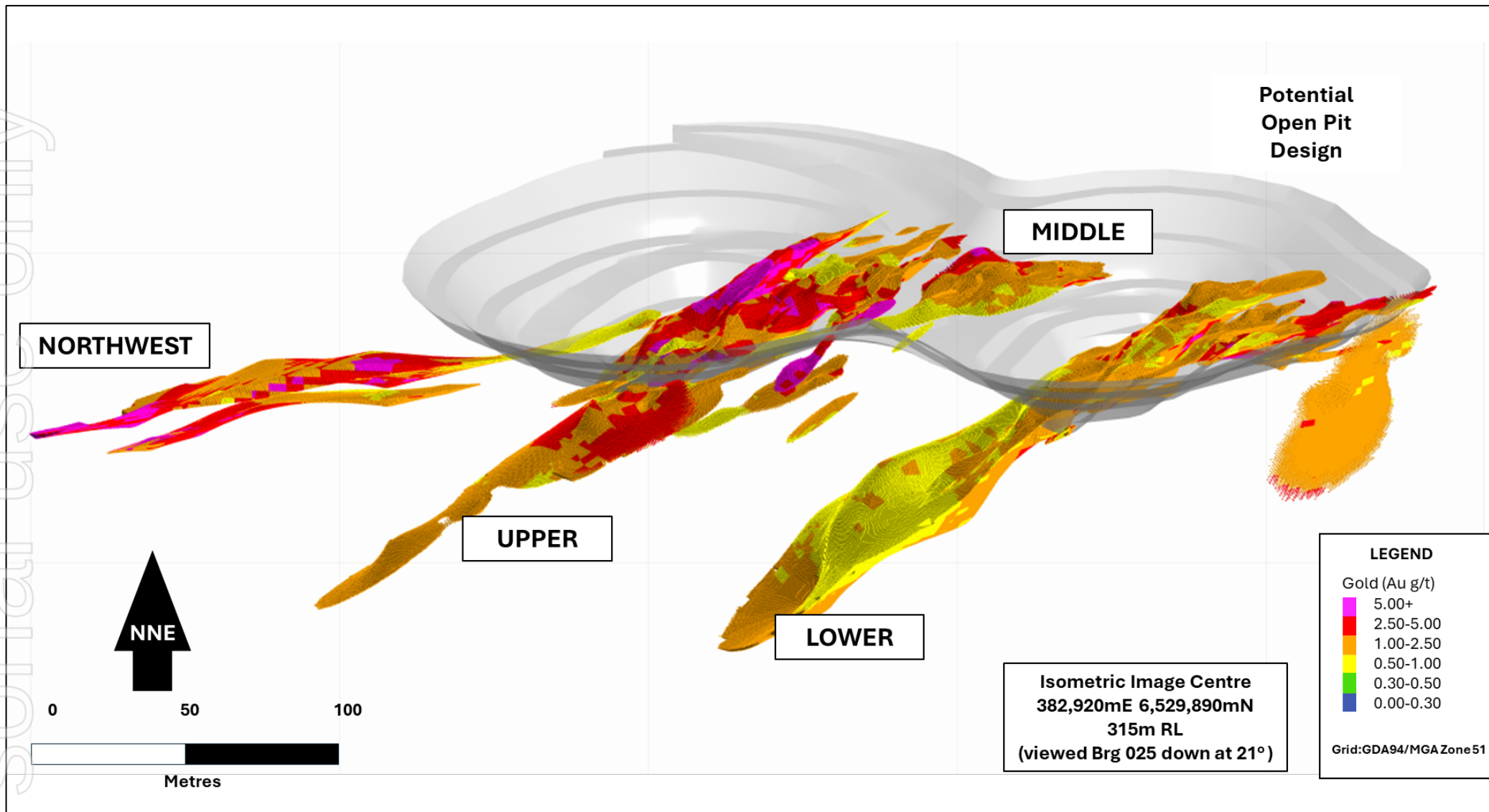
Figure 13: Isometric view, looking down and toward the NNE, of the Lady Herial gold deposit illustrating the Upper, Lower, Middle and Northwest Structures coloured by estimated gold grade (g/t Au).
