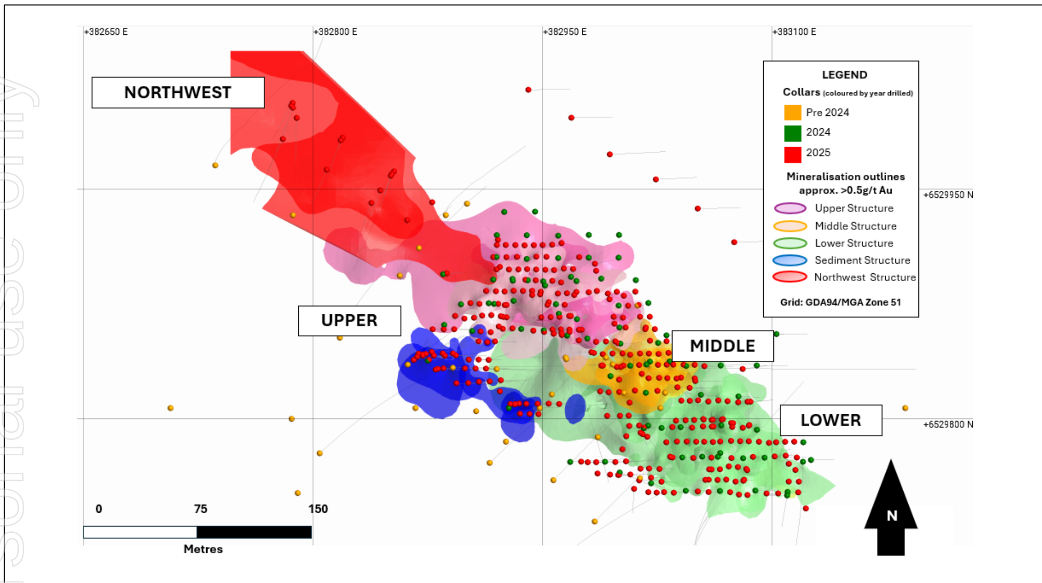
Figure 9: Plan View of the Lady Herial gold deposit illustrating the Upper, Lower, Middle and Northwest Structures and all drilling coded by period drilled.
