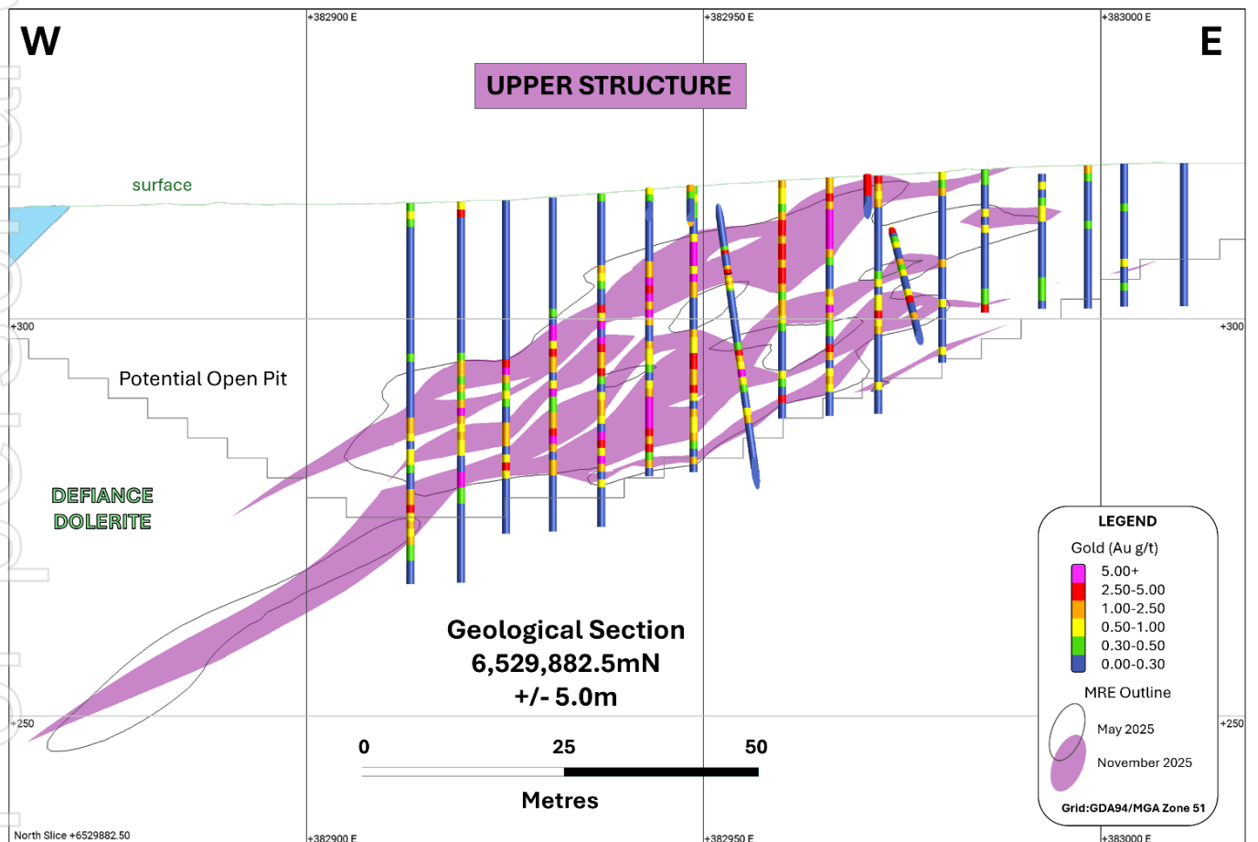
Figure 6: Geological cross section through the Upper Structure showing the current more discrete modelled high grade lenses against the 7 May 2025 MRE outline (with a potential open pit shell).
