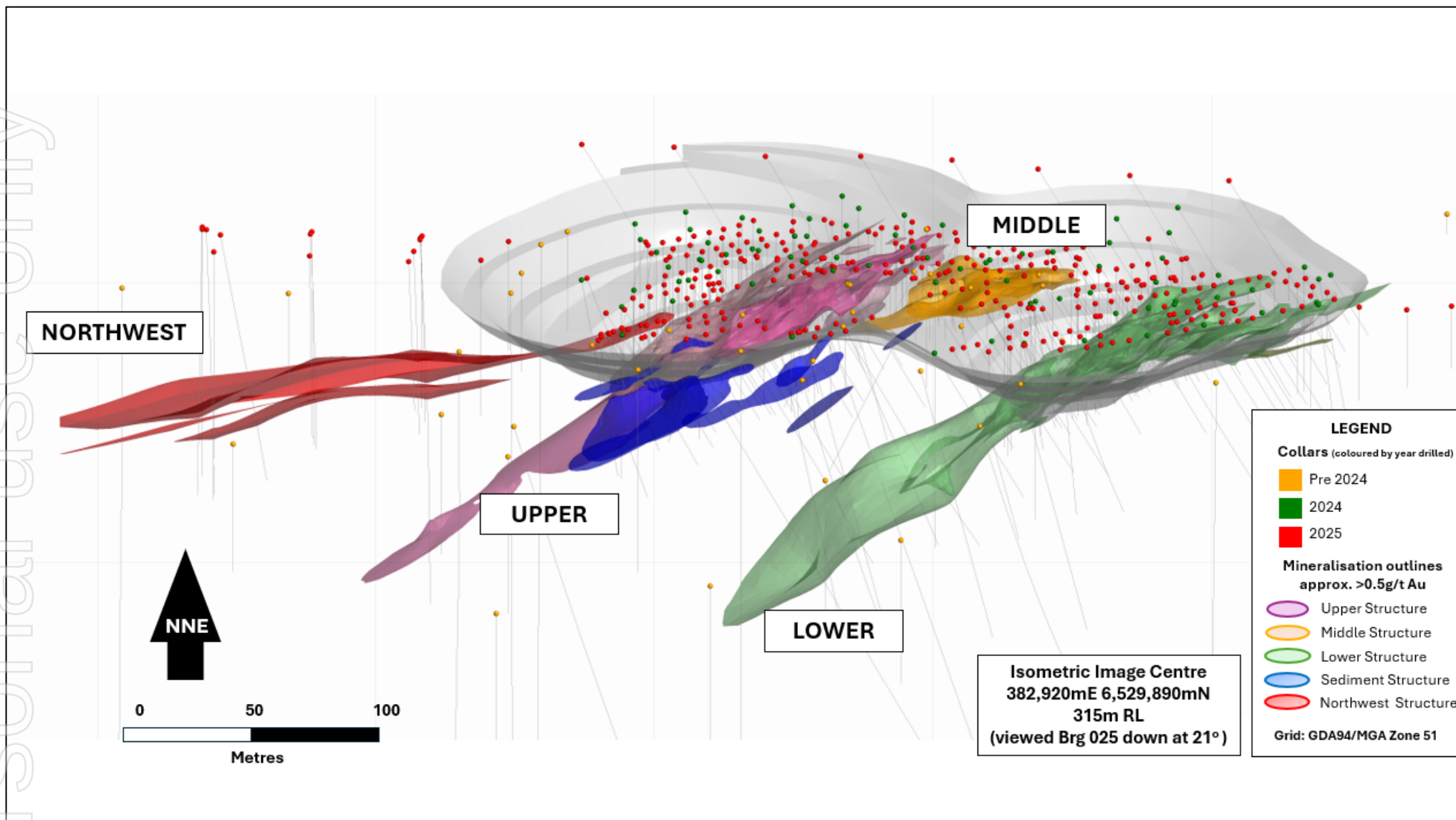
Figure 12: Isometric view, looking down and toward the NNE, of the Lady Herial gold deposit illustrating all drilling coded by period drilled and a potential open pit design.
