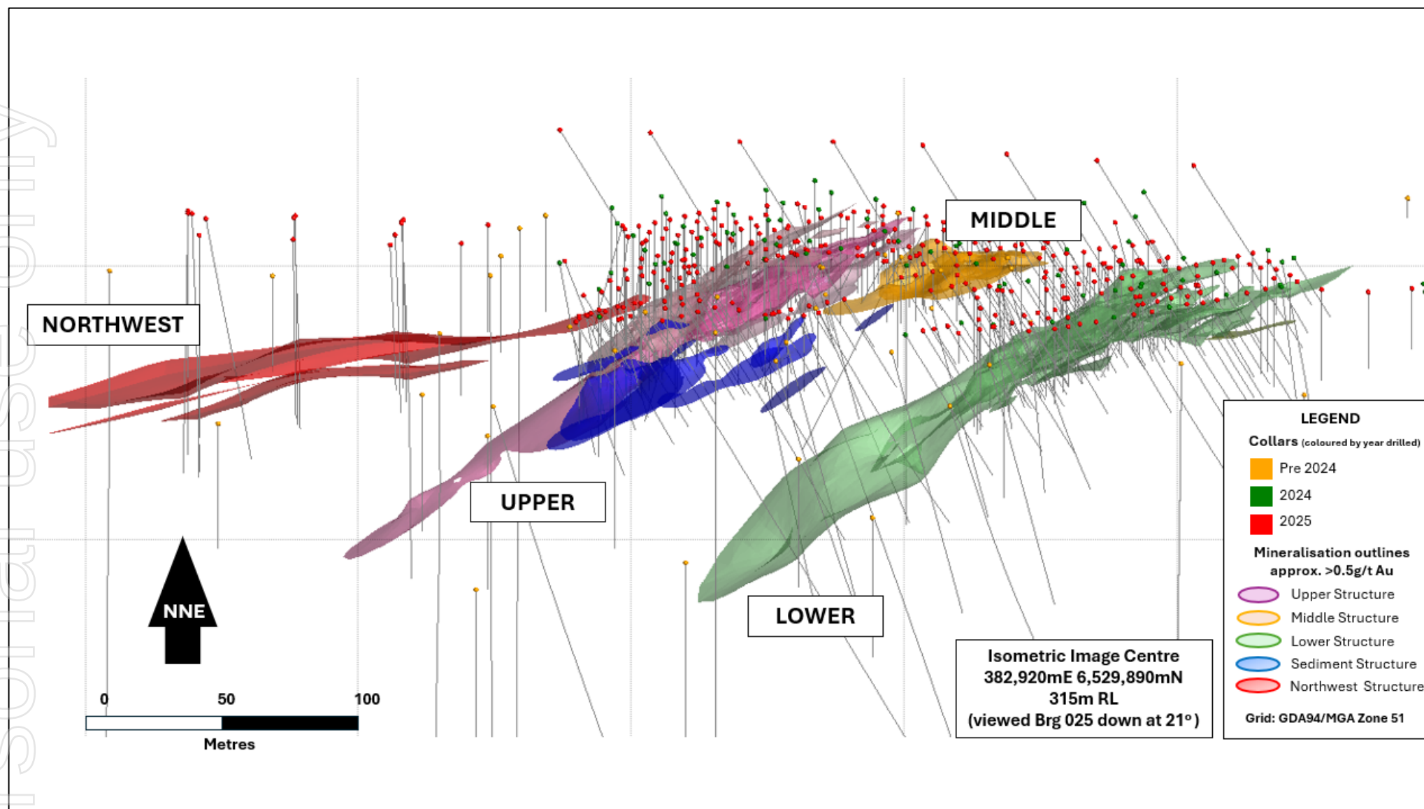
Figure 11: Isometric view, looking down and toward the NNE, of the Lady Herial gold deposit illustrating the Upper, Lower, Middle and Northwest Structures and all drilling coded by period drilled.
