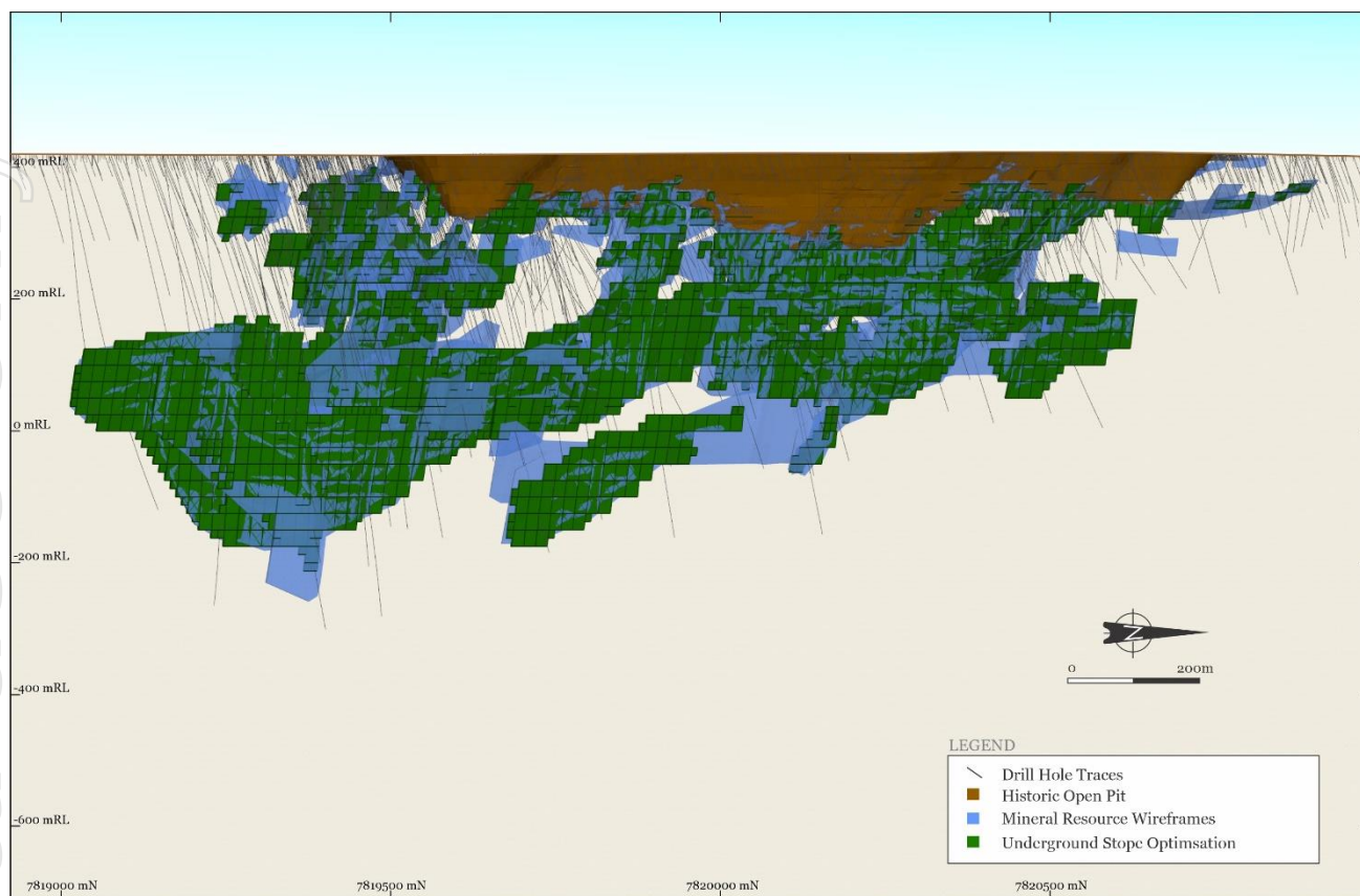
Figure 3 – Groundrush Gold Deposit
