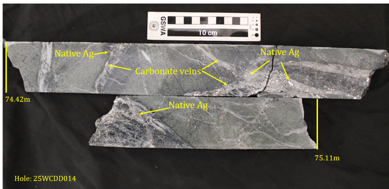
Figure 4. Photograph of cut half HQ3 drill core (25WCDD014) from 74.42m to 75.11m showing 1% visually estimated, 2mm to 4mm long native silver grains hosted within and adjacent to 1cm to 3cm thick carbonate veins in an ultramafic host rock.
