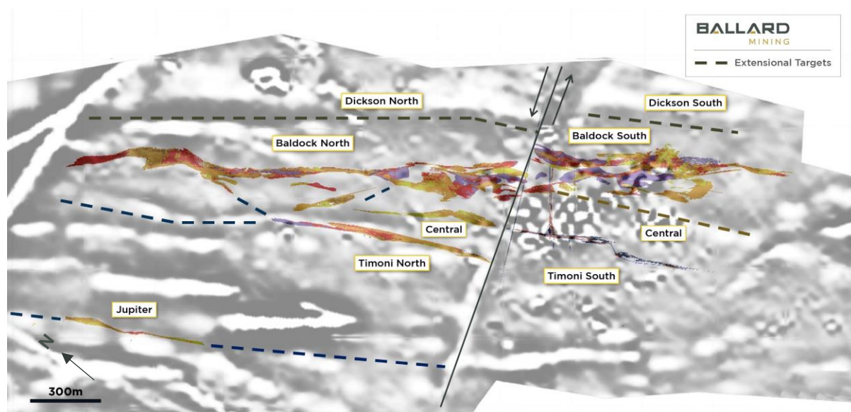
Figure 3 - Plan view of the Baldock gold deposit showing major lodes, faults and mineralised trends,
