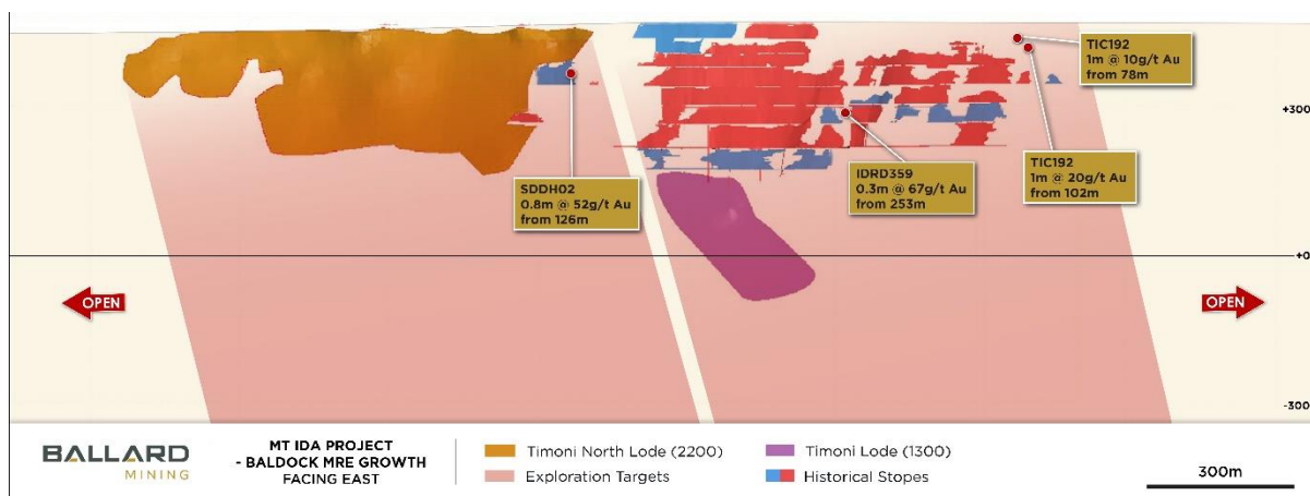
Figure 5 - Long section showing the Timoni deposit, deeper drilling results and Exploration Target. The size and grade of the October 2025 Exploration Target is conceptual in nature. There has been insufficient exploration to estimate a Mineral Resource, and it is uncertain if further exploration will result in the estimation of a Mineral Resource.
