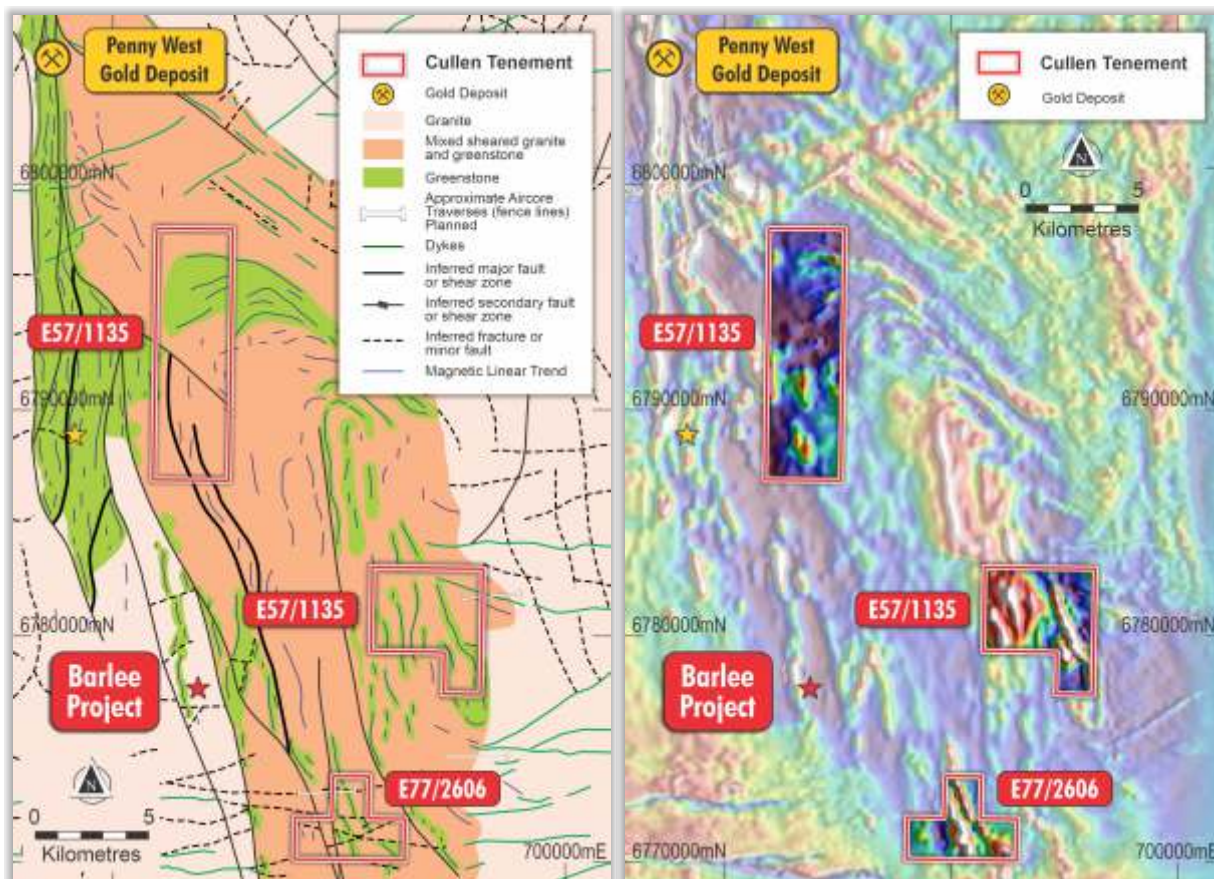
Geology Map and Lithium Prospectivity (aerial mag image)
