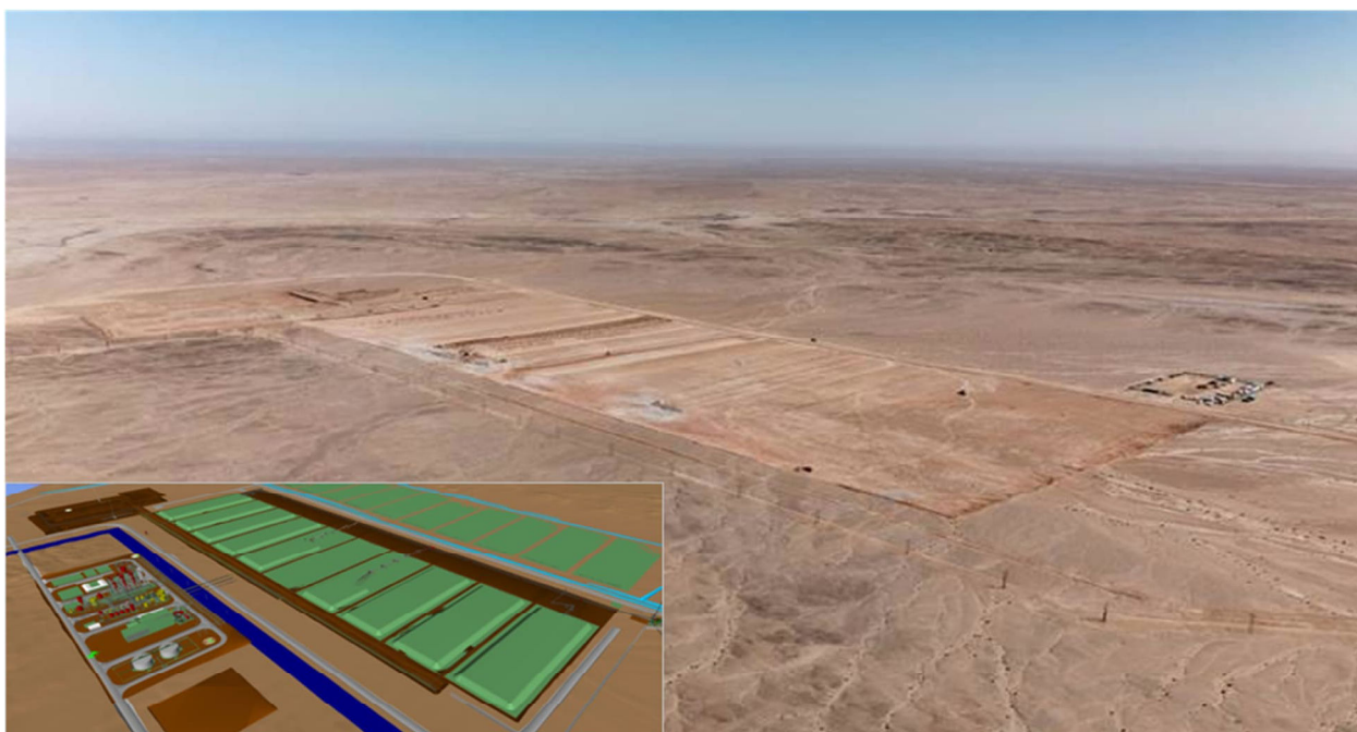
Figure 3: Heap leach pad earthworks advancing strongly (inset: 3D rendering of plant design from same perspective)
