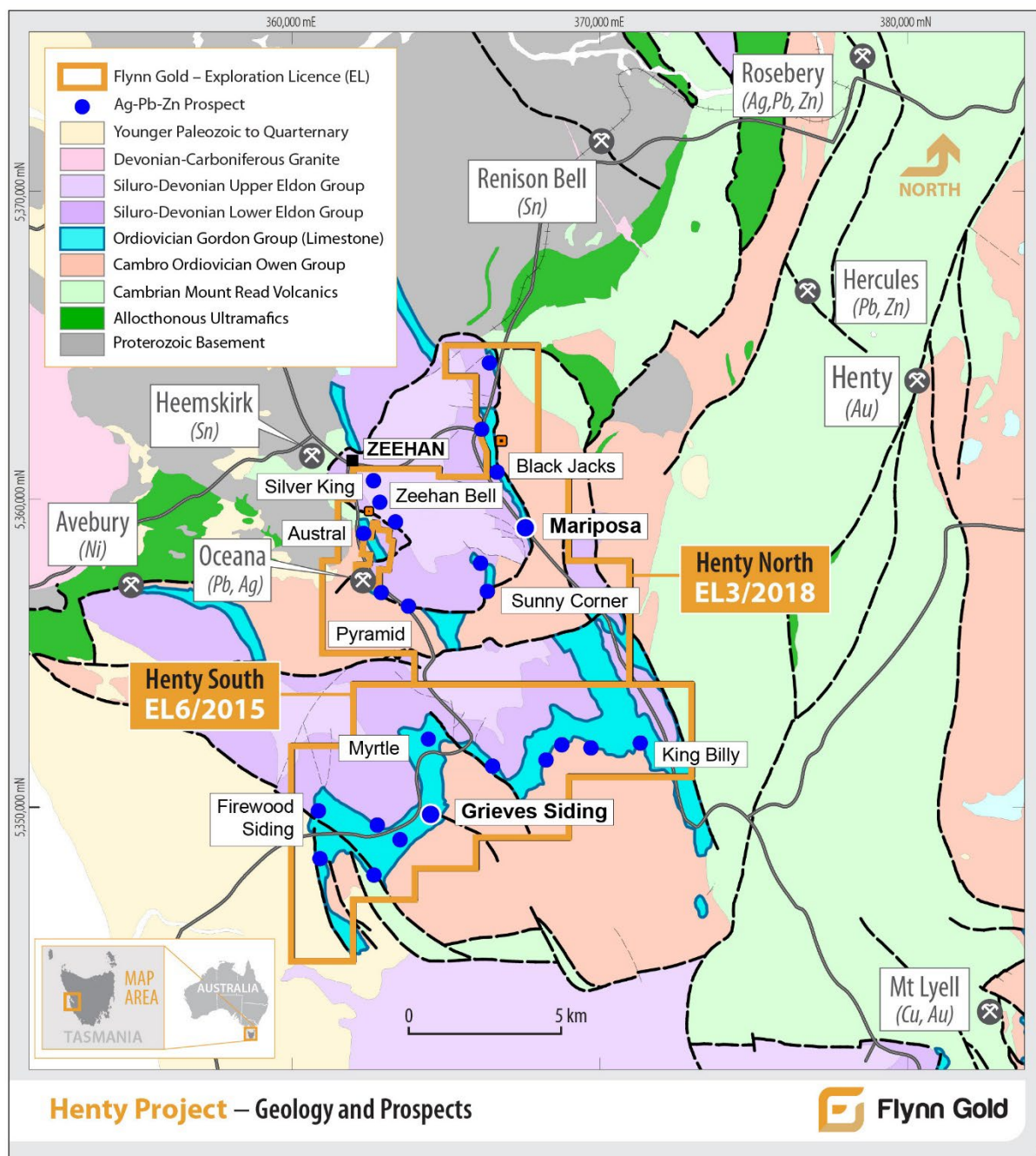
Figure 3 - Henty Project Geology and Silver-Lead-Zinc Prospects.
