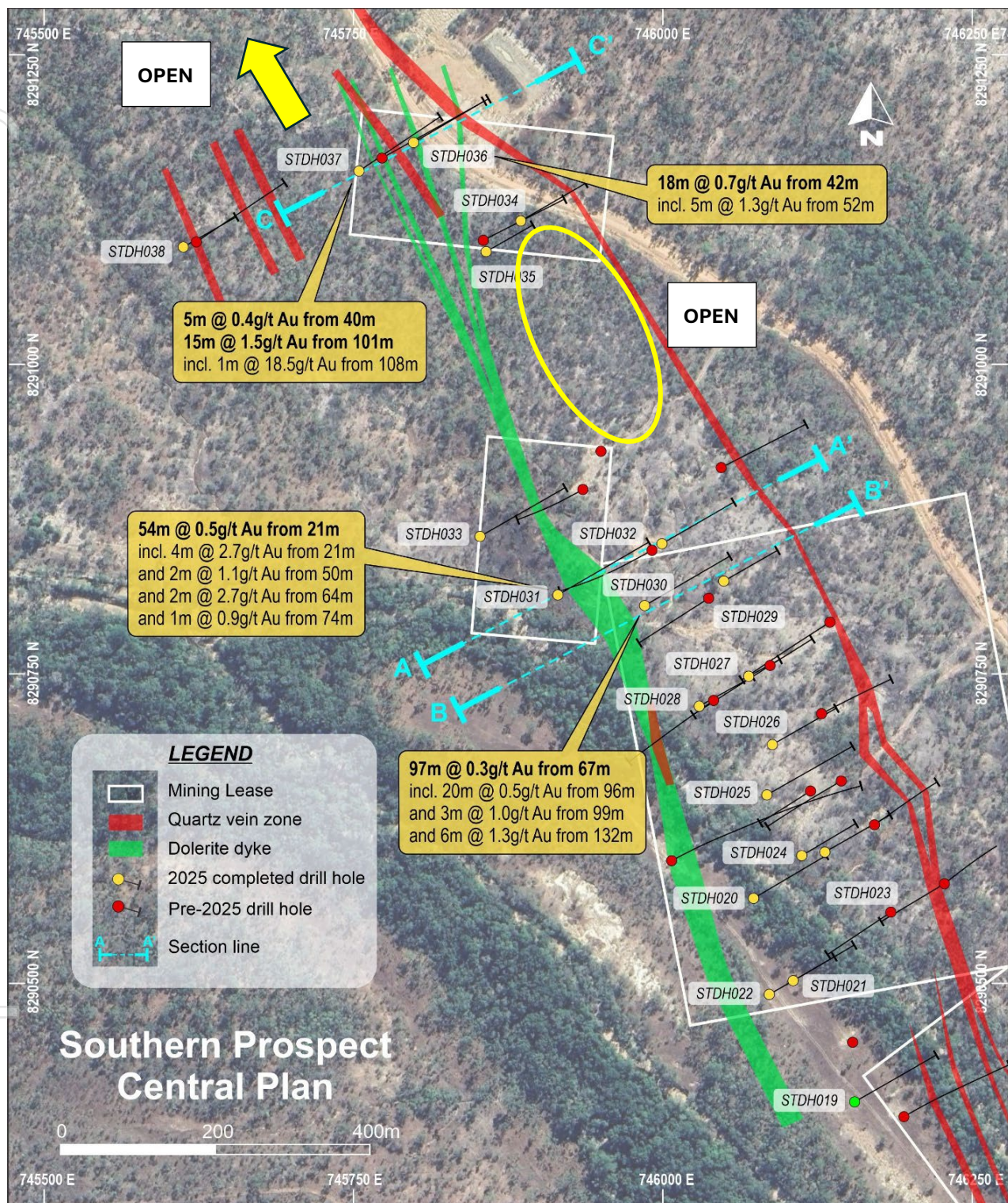
Figure 1: Southern Target plan view showing recently completed RC collars and previous drill sites, a large open area of mineralisation is still to be drill tested to the north west and up to the central zone
