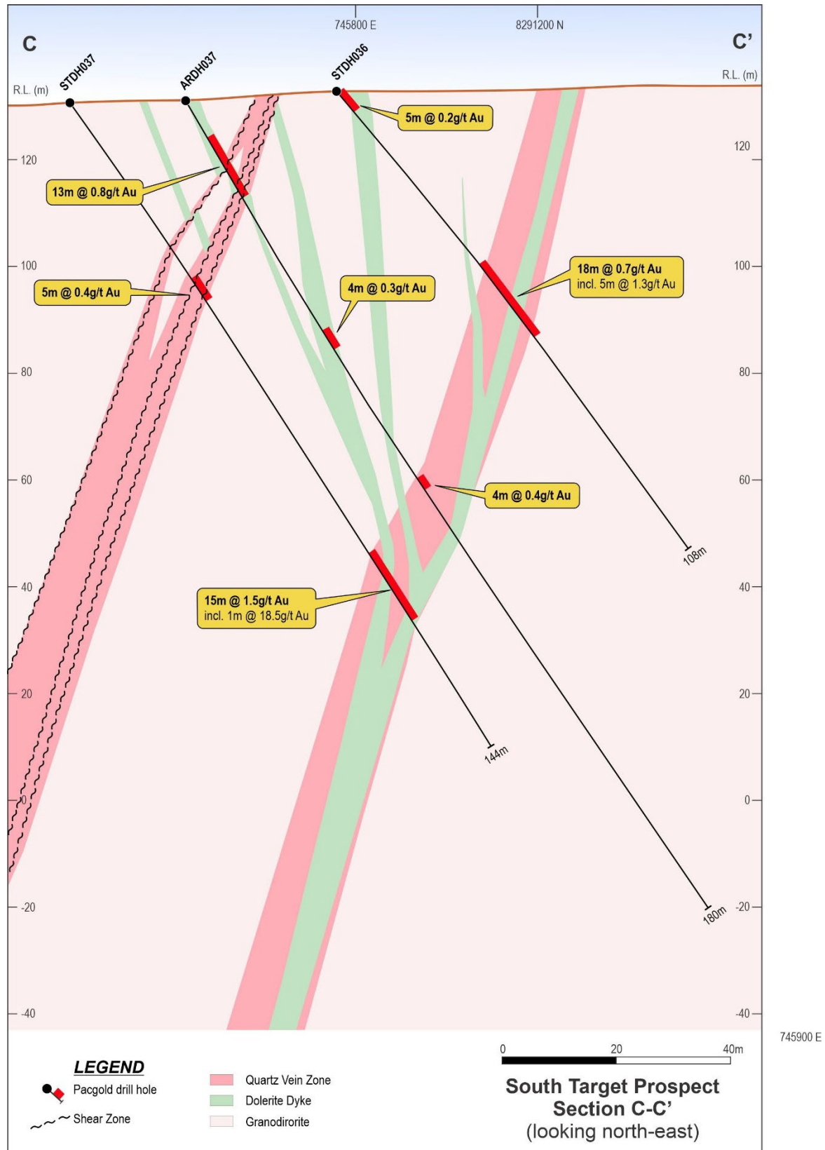
Figure 3: Section C-C' through Southern Target area with historic and new drilling
