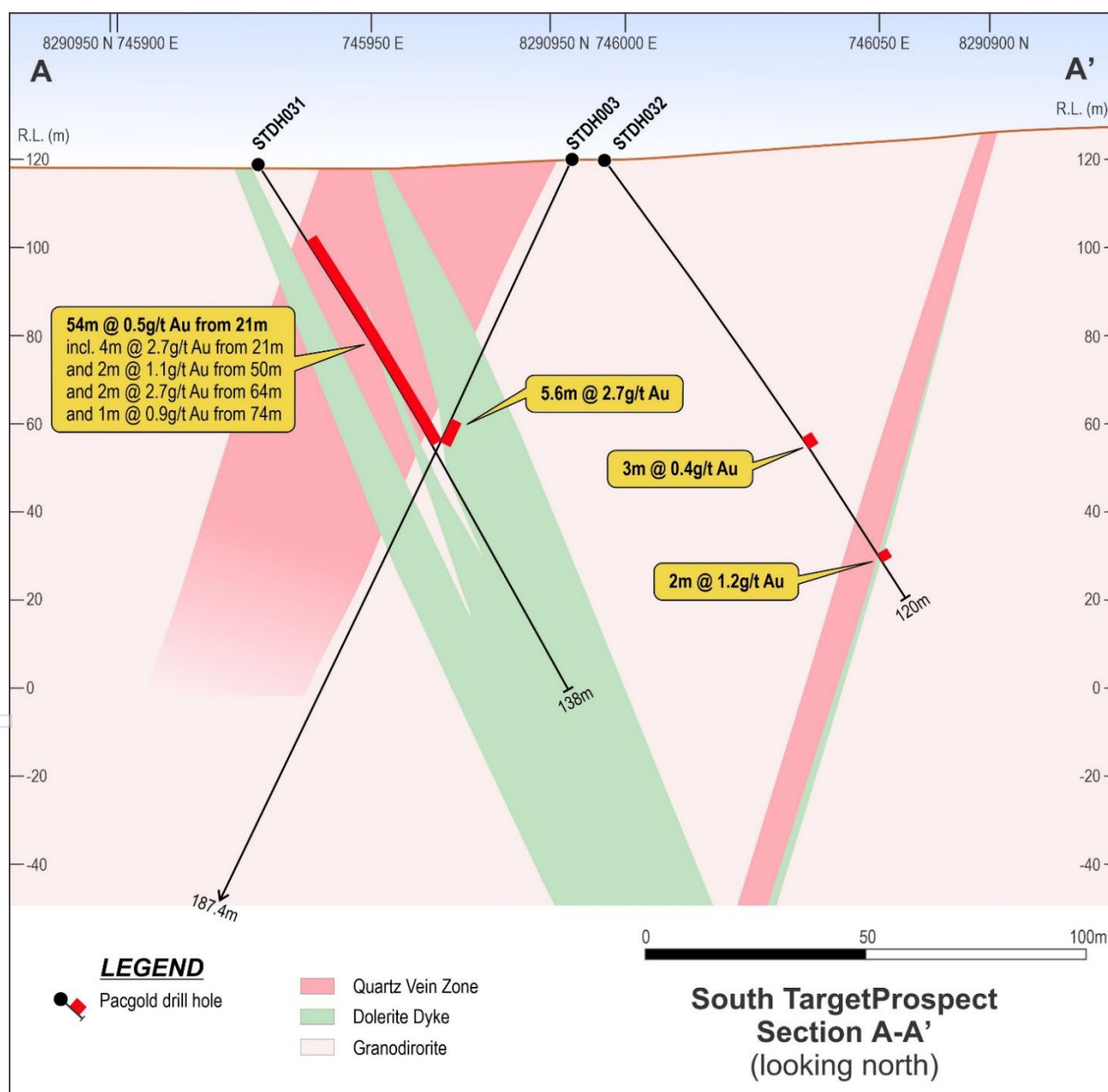
Figure 1: Section A-A' through Southern Target area with historic and new drilling
