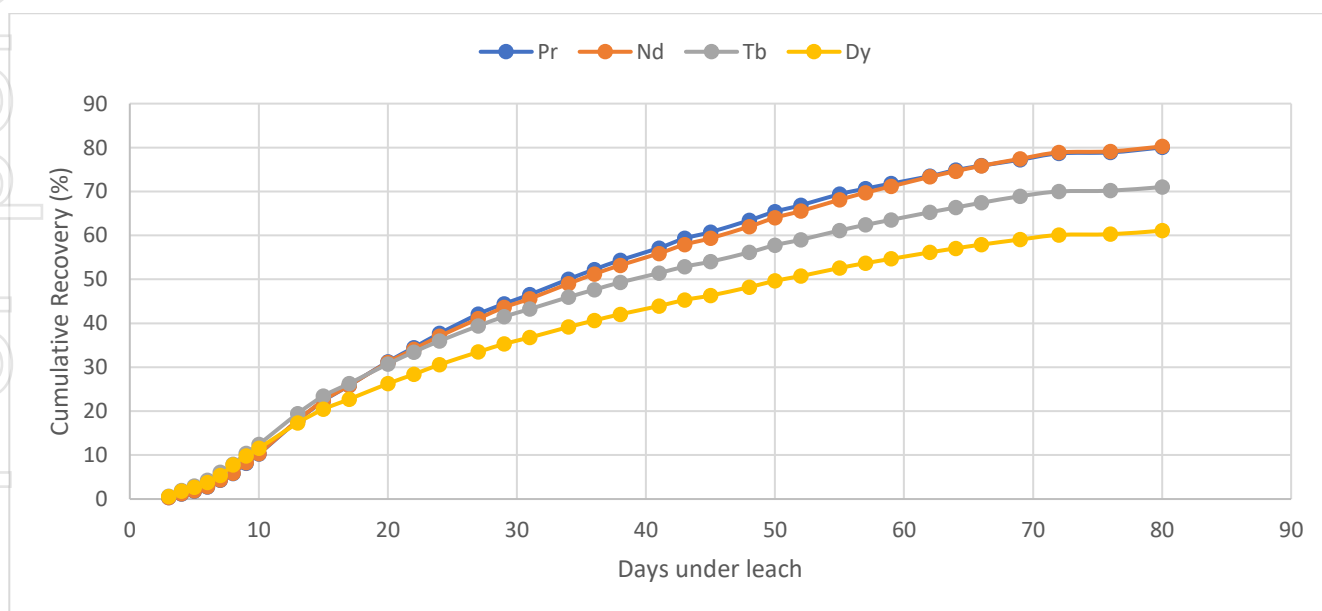
Figure 3: Inside Centre Composite Heap Leaching Results – Cumulative Recovery by Day
