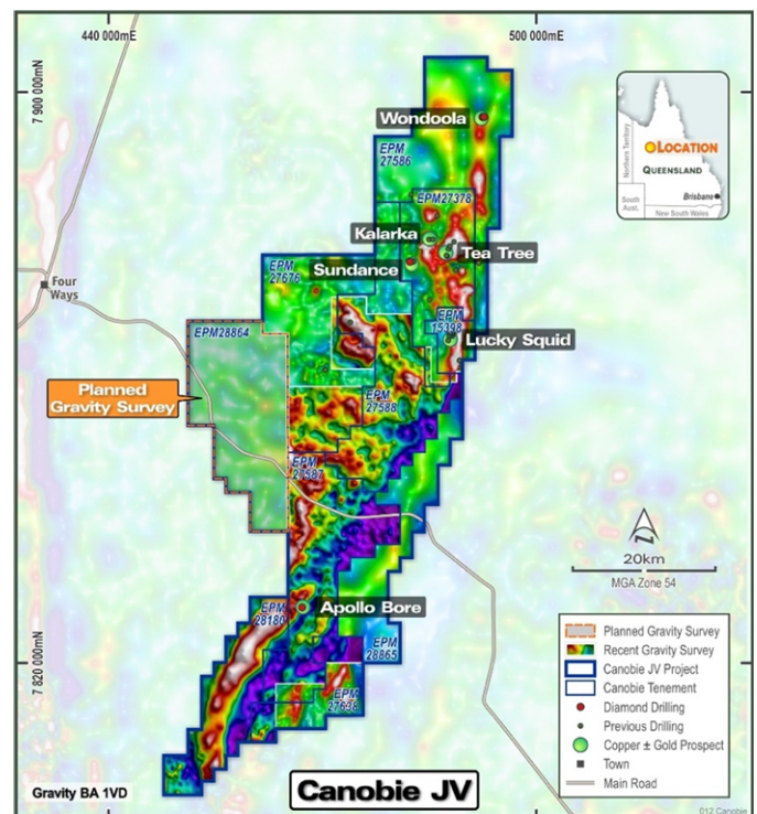
Figure 1: Canobie Project area showing gravity survey
