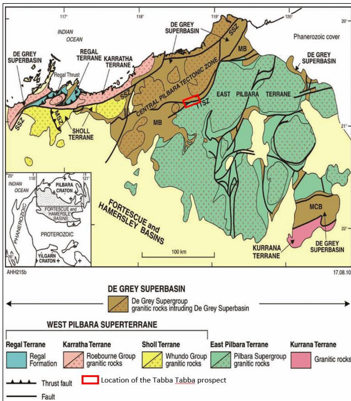
Figure E.6. Simplified geology of the northern Pilbara Craton (adapted from Hickman and Van Kranendonk, 2012), highlighting the location of Tabbatabba within the craton.
