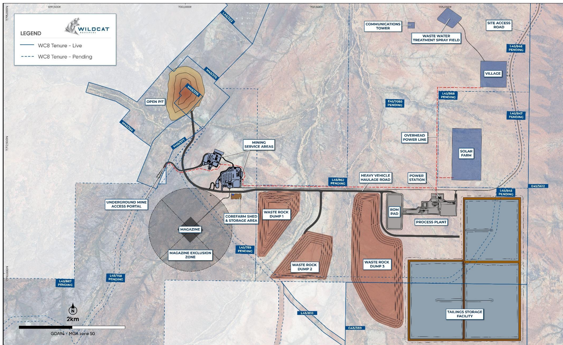
Figure E.28 Project Site Layout
