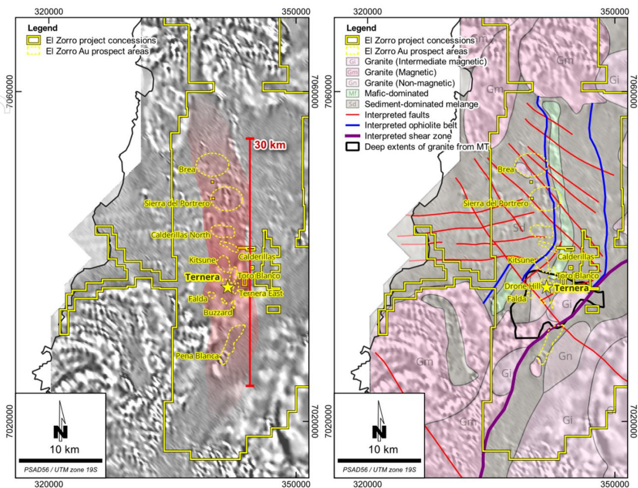
Figure 7: El Zorro Gold project regional airborne magnetic geophysics data imaging and interpretation: Example of reprocessed and filtered regional government AMAG survey data overlain by El Zorro gold prospects and El Zorro gold corridor (red shaded area) (left), and high-level interpretation using airborne magnetic survey images (right), which has identified multiple late-Triassic to early-Jurassic aged granitic intrusions and contacts with older metasediments and metavolcanic host rocks, and this regional bedrock interpretation is assisting the company with gold targeting along a well-defined north-south corridor. Refer to ASX announcement dated 2 April 2025.
