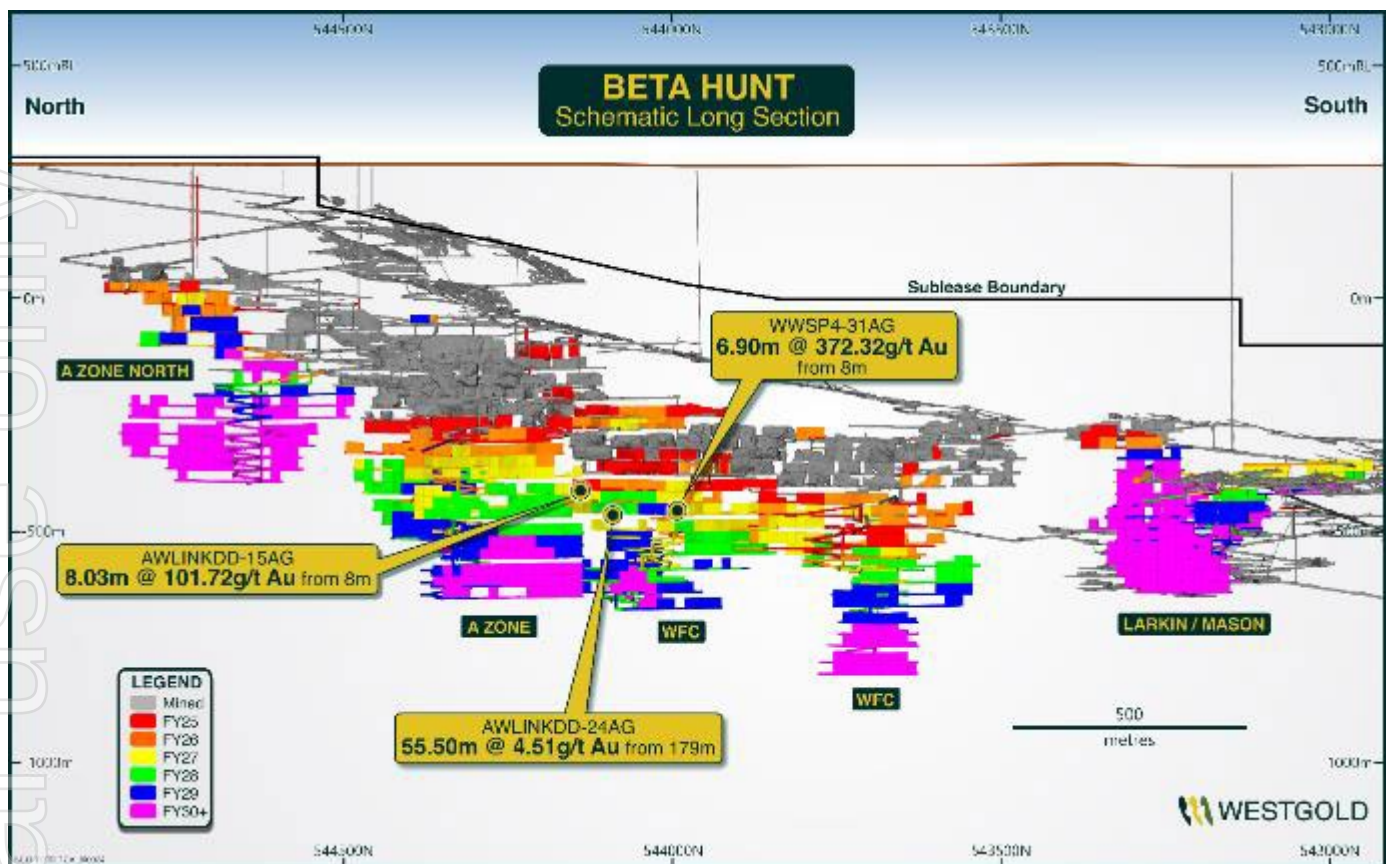
Figure 11: Beta Hunt FY25 Life of Mine plan schematic long-section: select drill results returned in Q4 FY25
