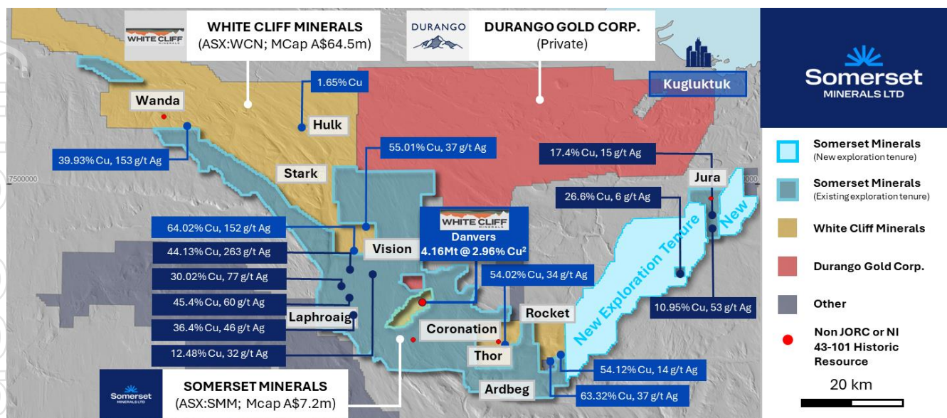
Figure 5: Regional overview showing Somerset's extensive landholding in the Coppermine region & previous rock chip results 2 . Mcap as at 09/05/2025.
