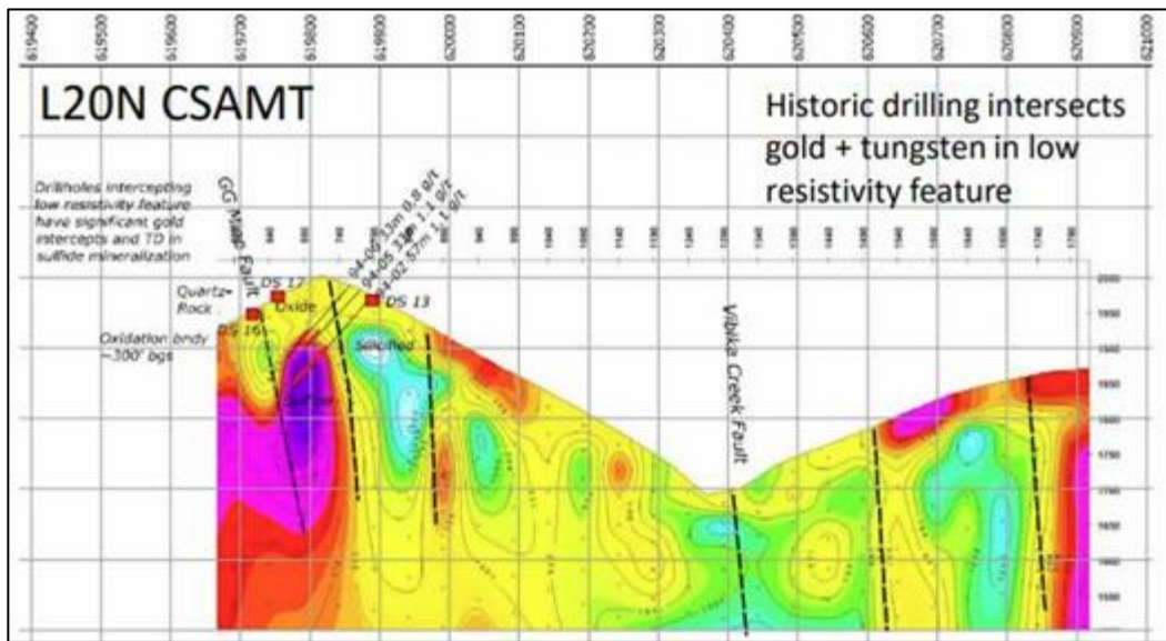
Figure 10: False-colour CSAMT cross section, Line 20N, where purple>red>orange are areas of relatively high resistivity, and where green<blue<white are areas of relatively low resistivity. The cross section shows the drill hole projection of drill holes 94-06, 94-05 and 94-02, all of which host broad zones of gold mineralisation. Refer to Table 2 and Appendix B for drill hole details. Refer to Figure 9 that shows the location of the L20N CSAMT cross section in plan view. Also shown are known and interpreted faults, including the Golden Gate Mine and Vibika Creek faults.
