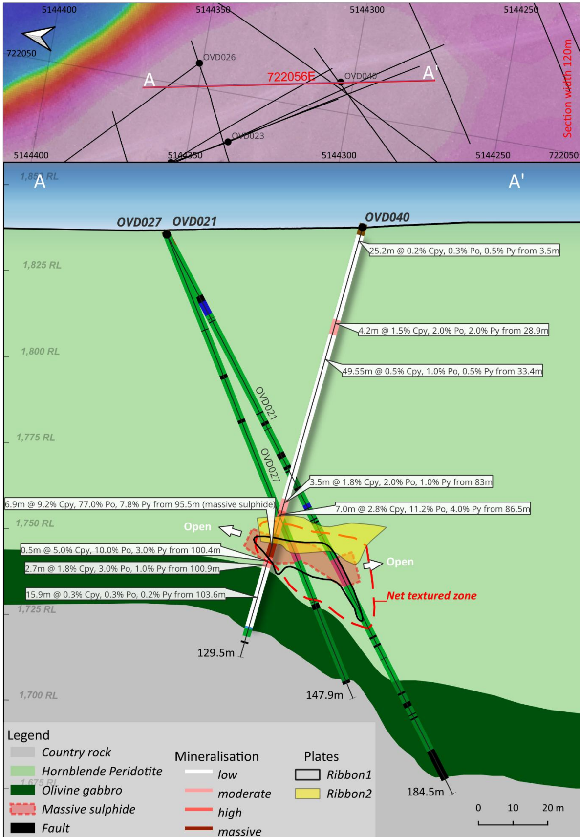
Figure 5. OVD040 cross-section of mineralised portion, looking to W¹¹
