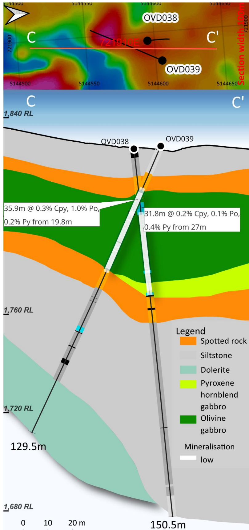
Figure 3. OVD038 & OVD039 cross-section of mineralised portion, looking to W 6
