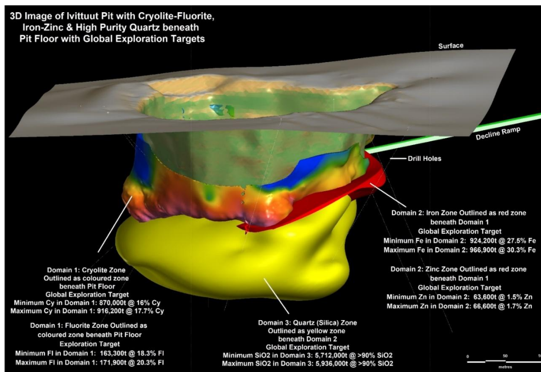
Figure 3: 3D oblique image showing domains 1&2 and high-grade quartz in domain 3
