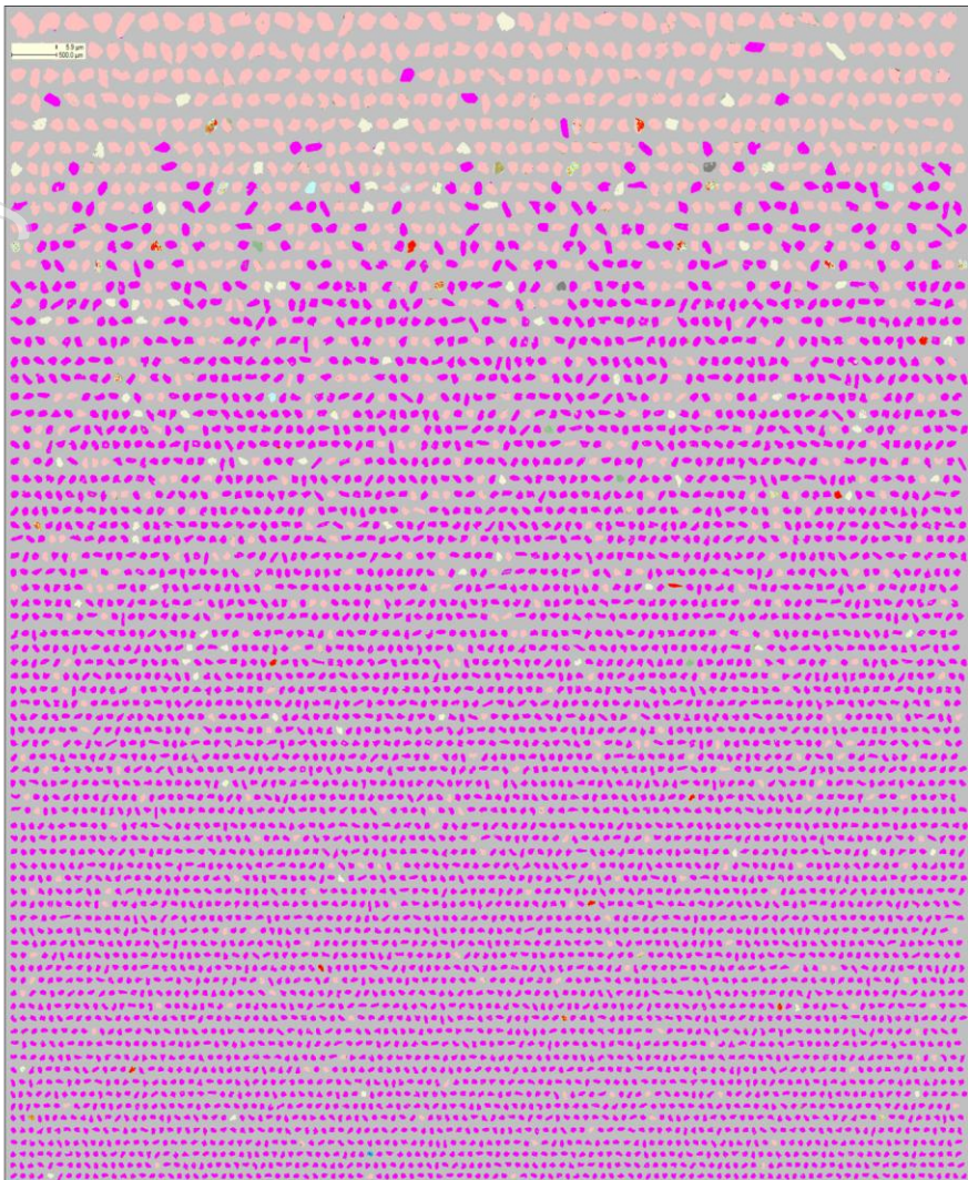
FM07: Zircon
