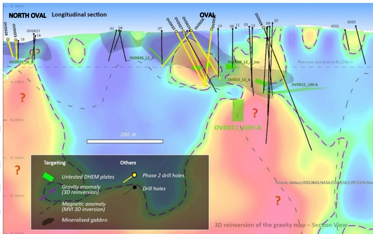
Figure 3. Longitudinal Section of 3D inversion of gravity survey
