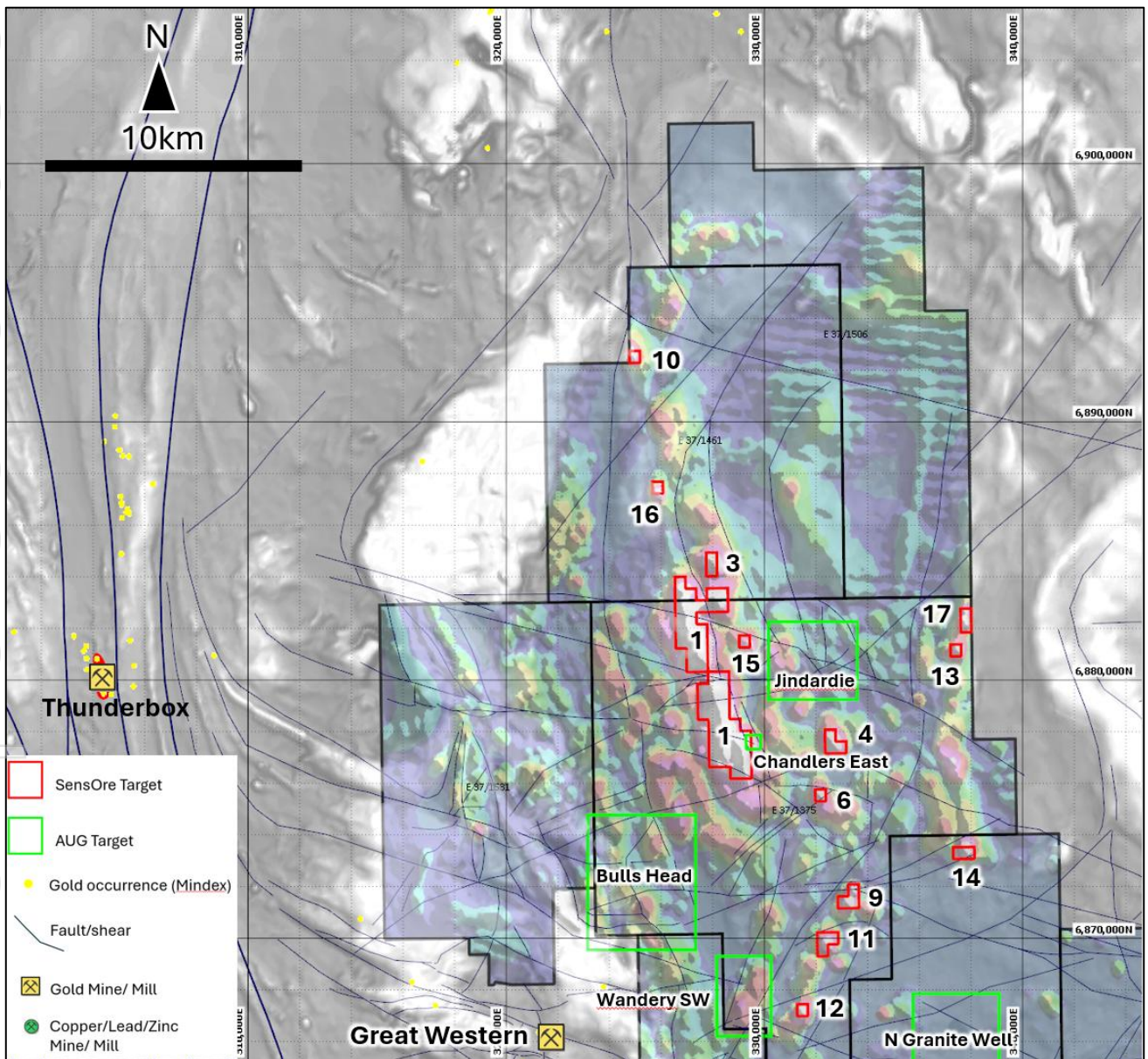
Figure 5 Music Well Gold Project northern section, showing SensOre targets as red polygons overlain on probability image and draped on GSWA state TMI RTP magnetics.
