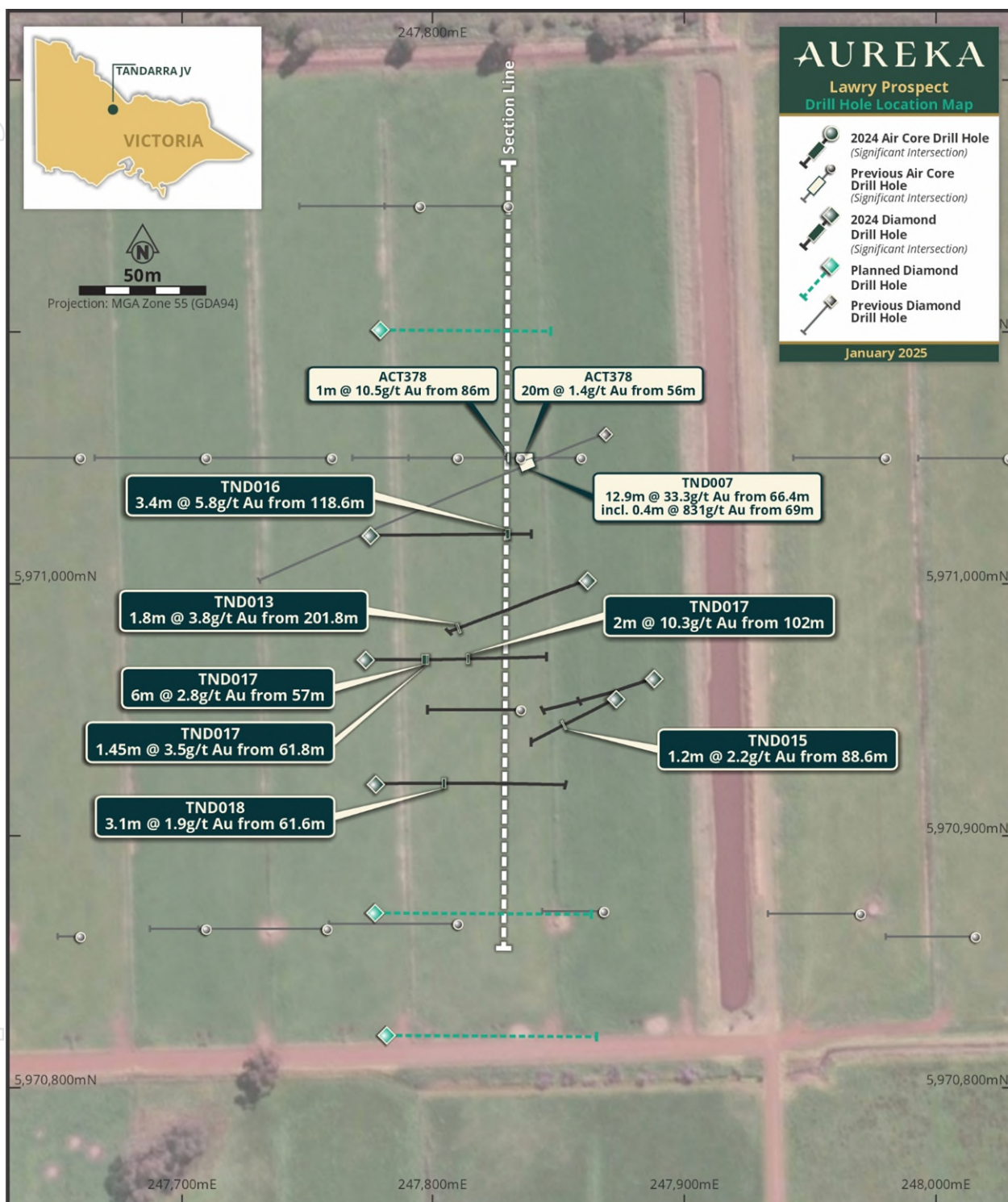
Figure 2 – Tandarra Gold Project - Lawry Prospect – depicting previous and a number of the current planned diamond drill holes.
