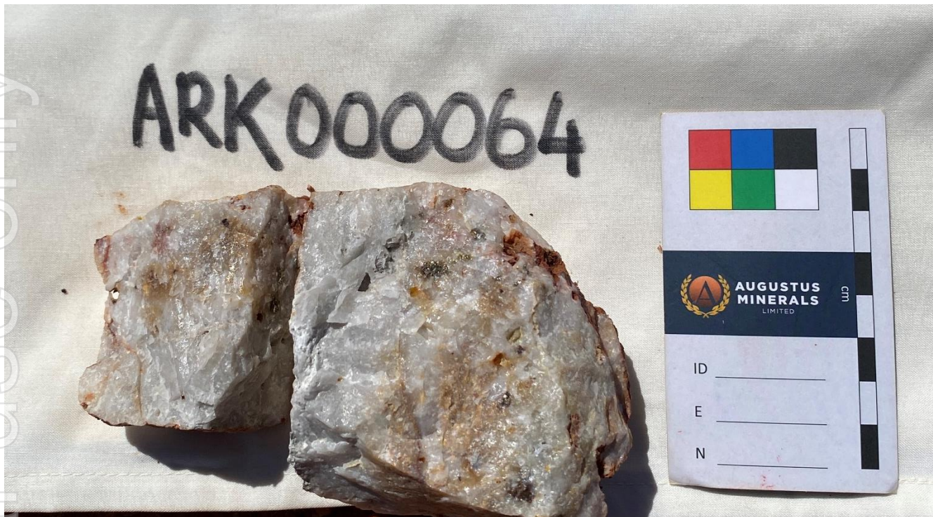
Figure 6 Photo of vein quartz from Augustus sample ARK000064 which assayed 50.1g/t Au at Clifton East. Note the brassy grey coloured fresh pyrite within the sample.
