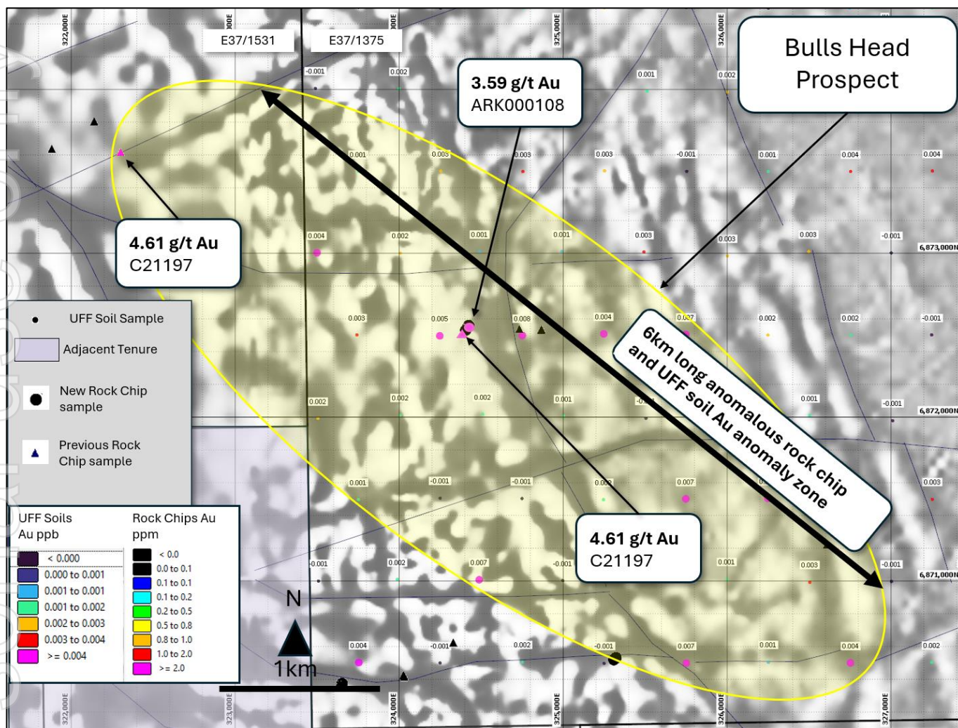
Figure 6 Rock chips and UFF soil samples (Au) at the Bulls Head prospect draped on an RTP 2VD magnetic image. Sampled quartz vein zone trends ENE and dips sub-vertically.
