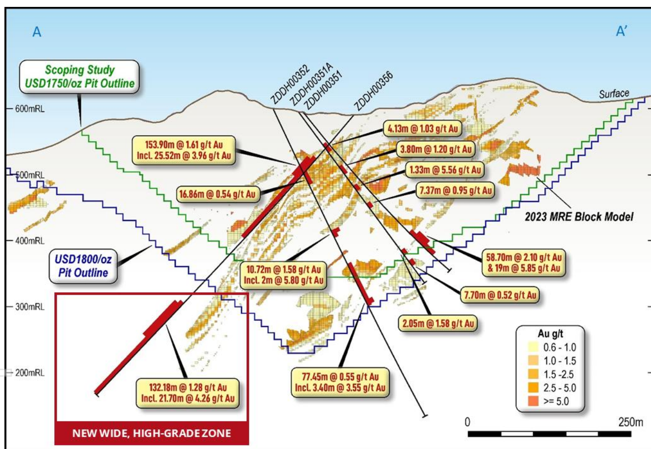
Figure 2: El Zorro Gold Project – Block Model Section (looking west): Hole ZDDH0356 shows new mineralised zone well outside of existing MRE. Block model shows indicated and inferred material >0.60g/t Au and is colour coded to Au g/t. Holes ZDDH0351 and ZDDH0351A projected onto section were drilled approximately 50m to the east.
