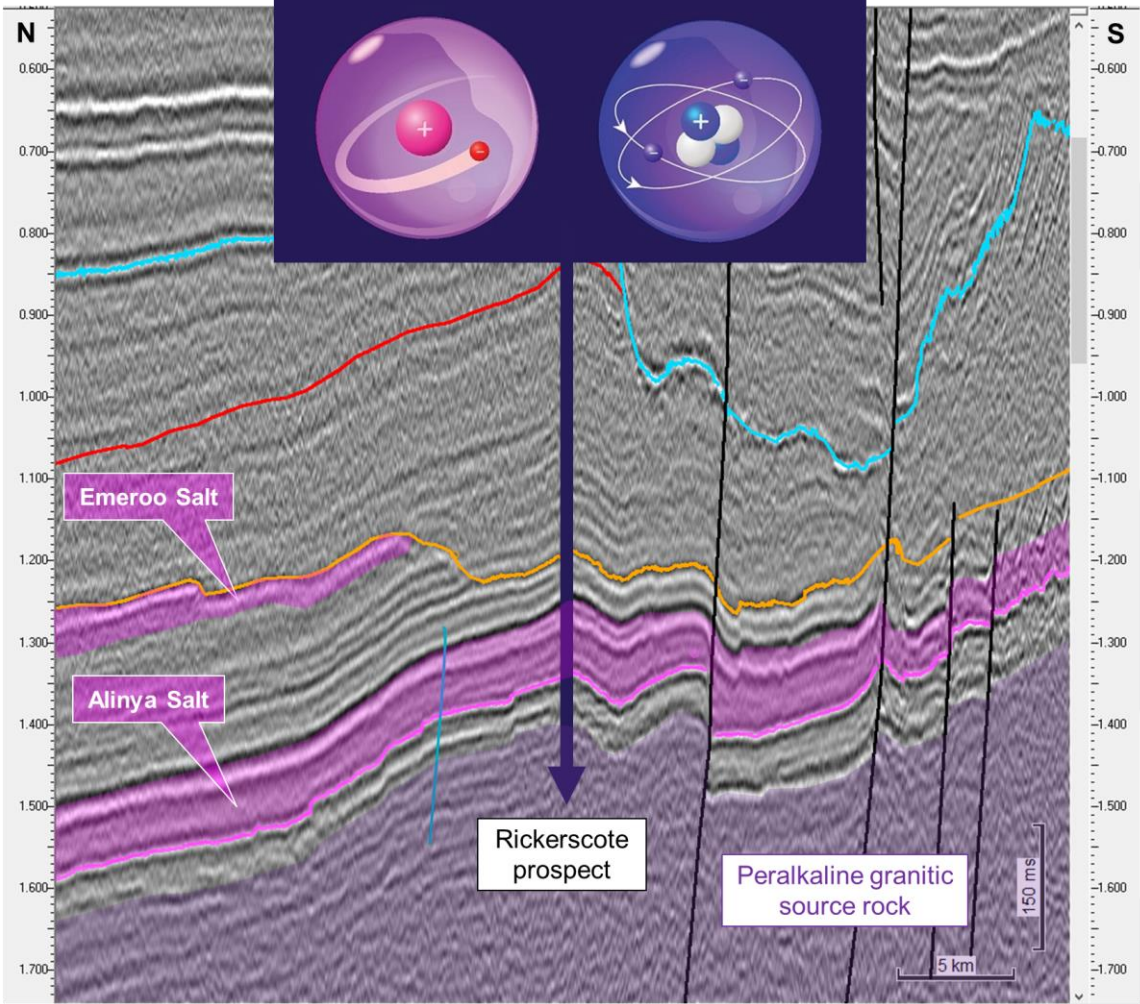
2D Seismic Line over Rickerscote Prospect
