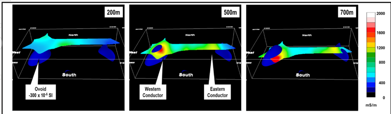
Figure 4: 3D perspective view looking north showing MLEM conductivity depth slices for MT Line A2 relative to the modelled reversely magnetised ovoid.
