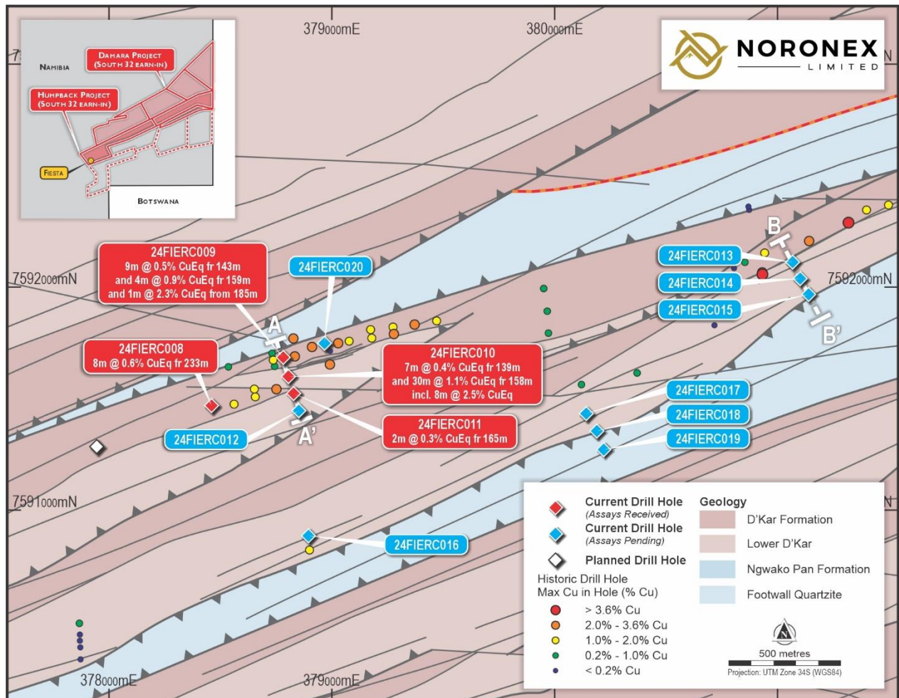
Figure 3: Drill locations and intercepts from the current drill program at the Fiesta Project.
