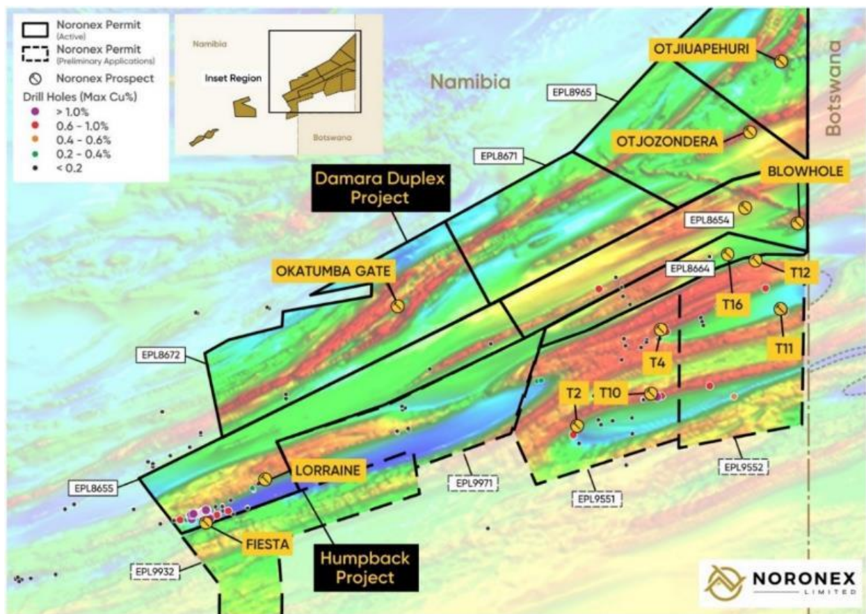
Figure 2: Regional aeromagnetic image of the Kalahari Copper Belt in Namibia with the current Noronex projects, showing Fiesta in the west and a number of magnetic complexes in the north at the Damara Project.
