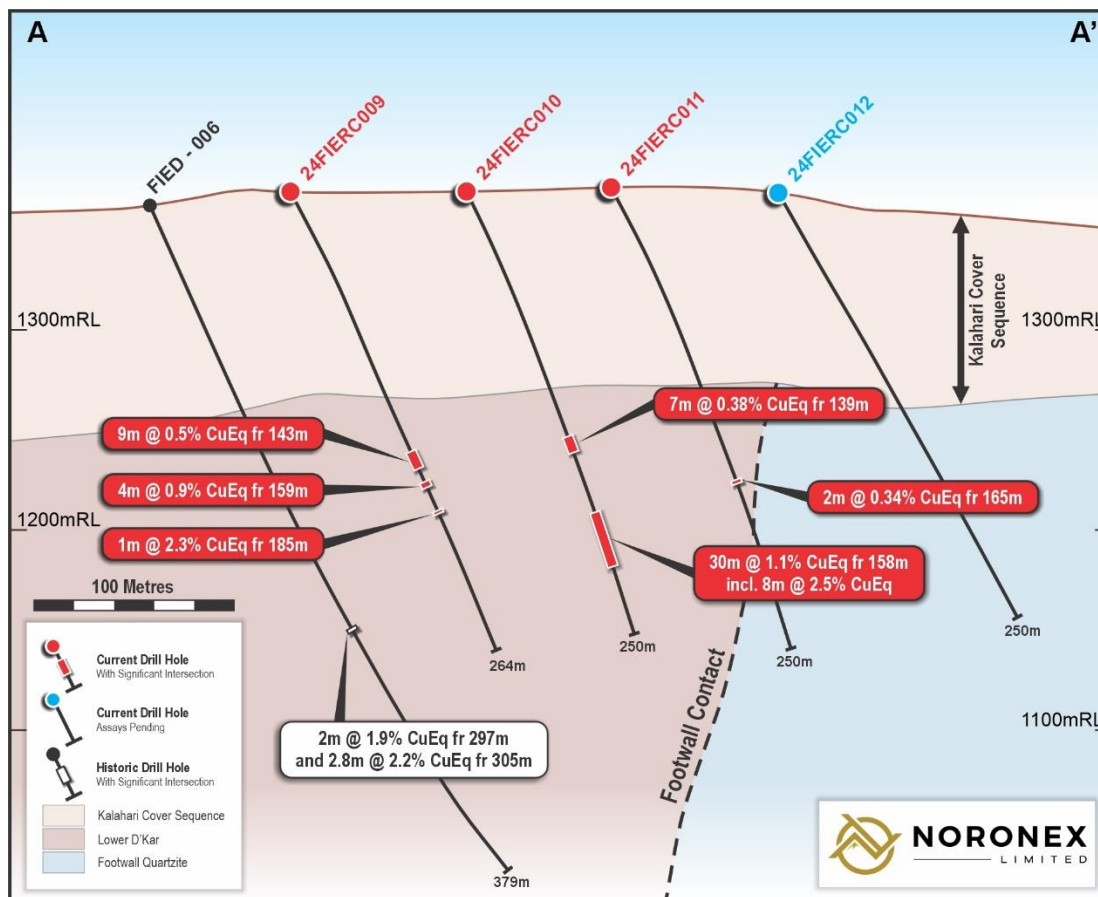
Figure 5: Drill section and intercepts from the current drill program showing north-south fence of holes at the Fiesta Prospect.
