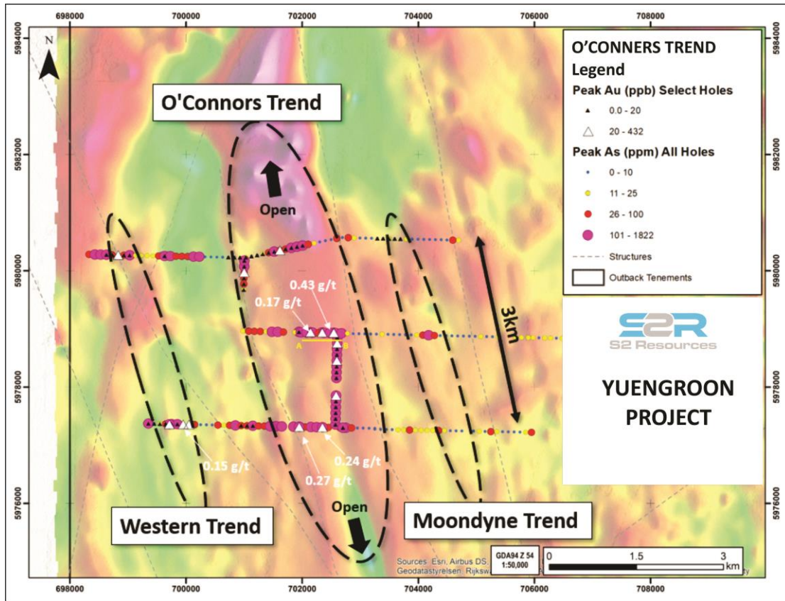
Figure 3: O'Connors aircore anomaly showing several trends with extensive arsenic-gold anomalism.
