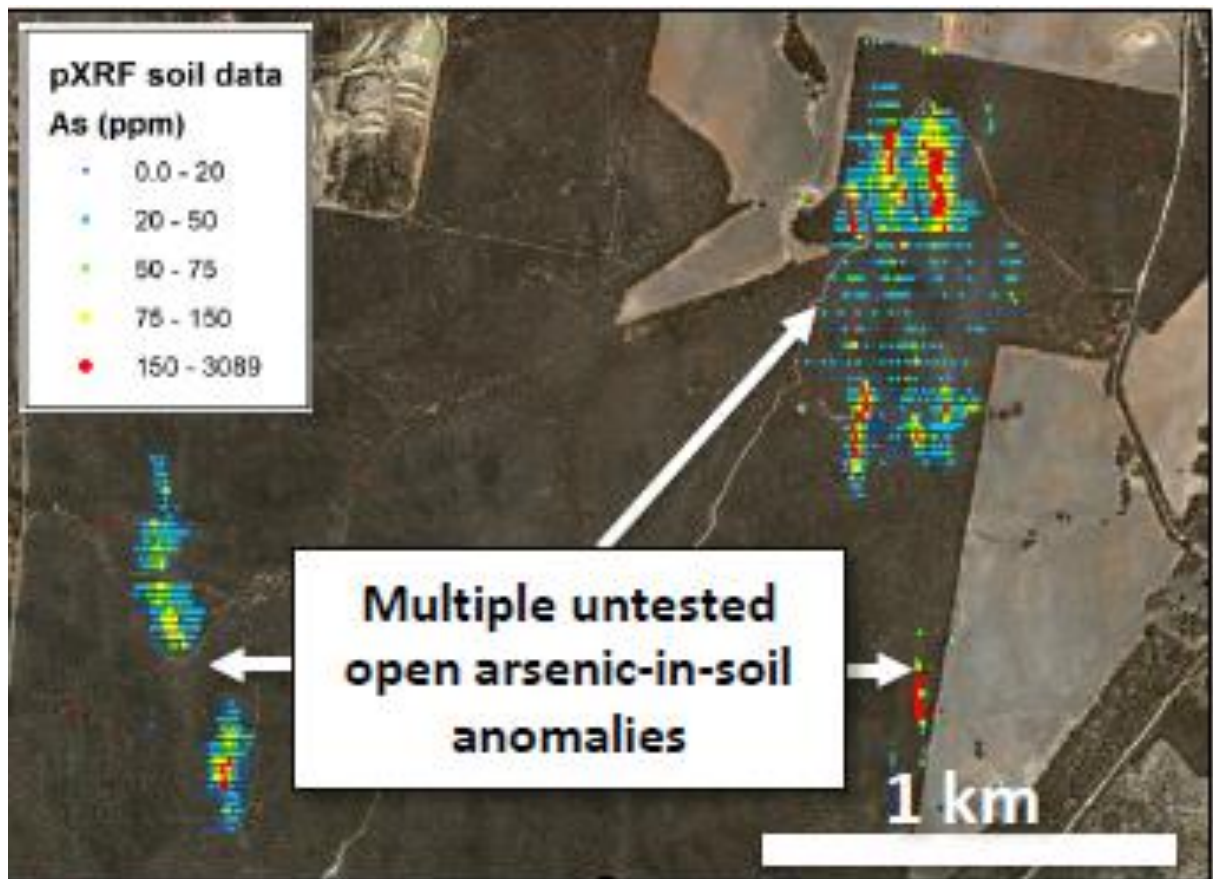
Figure 5: The Wedderburn soil anomaly showing several parallel arsenic anomalies.
