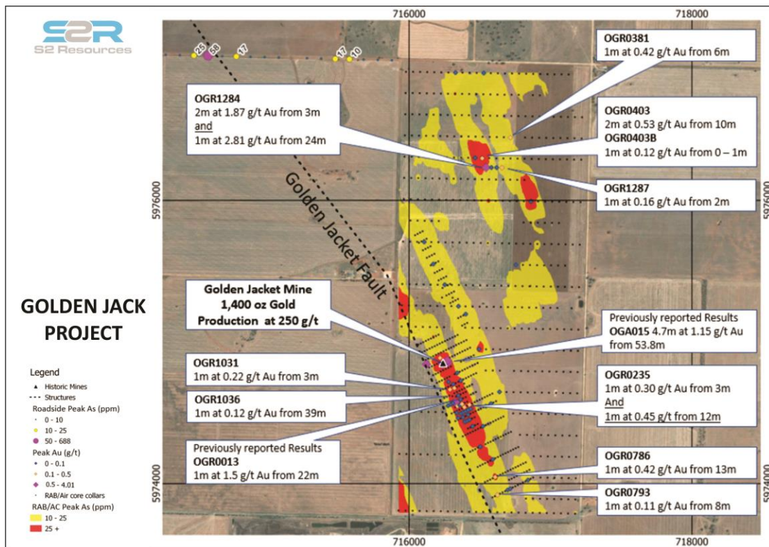
Figure 4: Golden Jacket aircore anomaly showing several trends anomalous in arsenic and gold.
