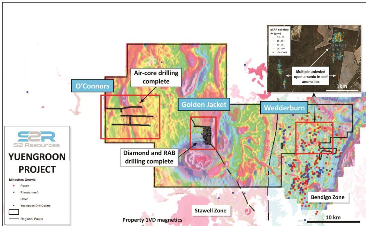
Figure 2: Overview map of the Yeungroon project showing location of gold-arsenic anomalies in soil sampling and aircore drilling undertaken by Valkea.
