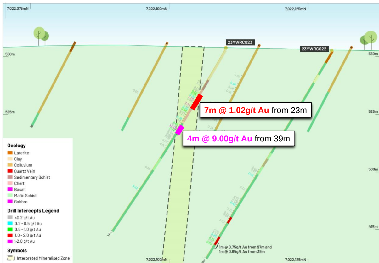
Figure 3: Cross section at Barwidgee Fault Prospect drilling.
