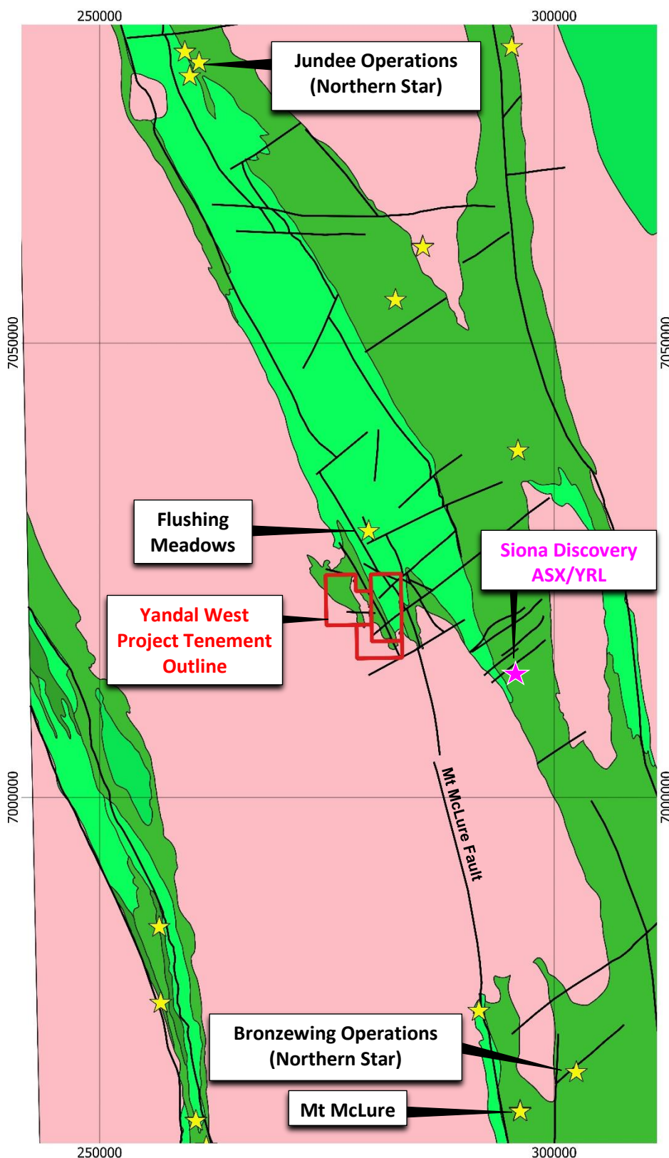
Figure 1: GSWA 1:2,500,000 bedrock geology map showing the location of the Yandal West Project on the Yandal Greenstone Belt and major gold mines and discoveries.
