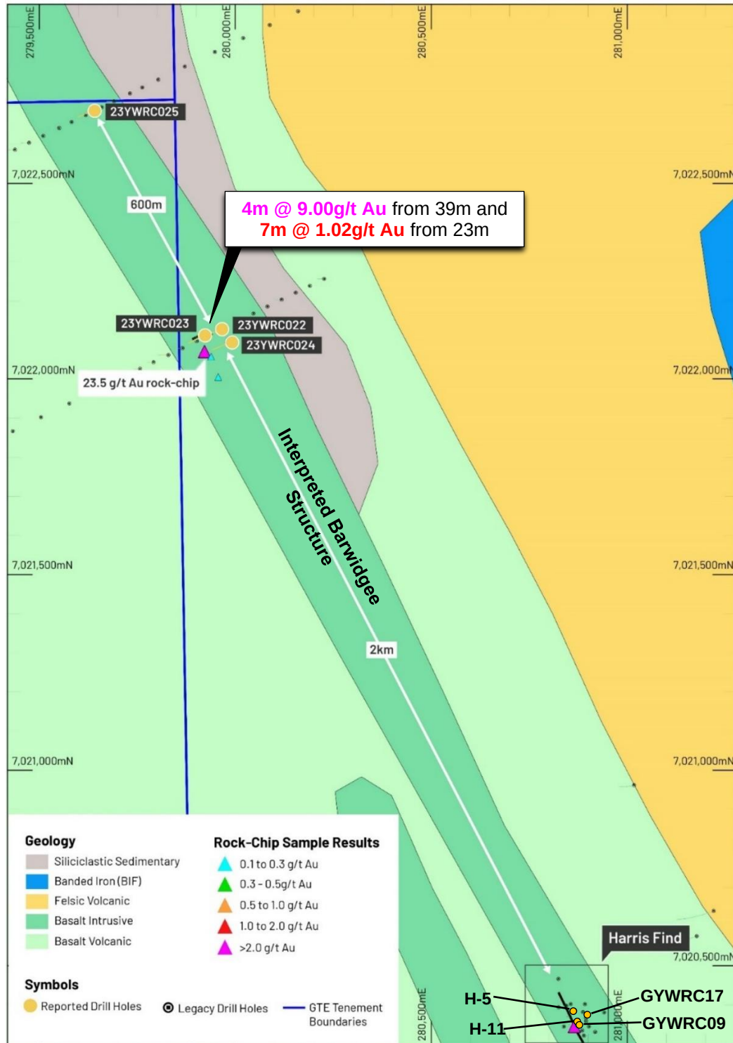
Figure 4: Drill collar locations along the Barwidgee Fault structure as well as significant rock assay results overlaid on Geological Survey of Western Australia 1:500,000 Geological Map
