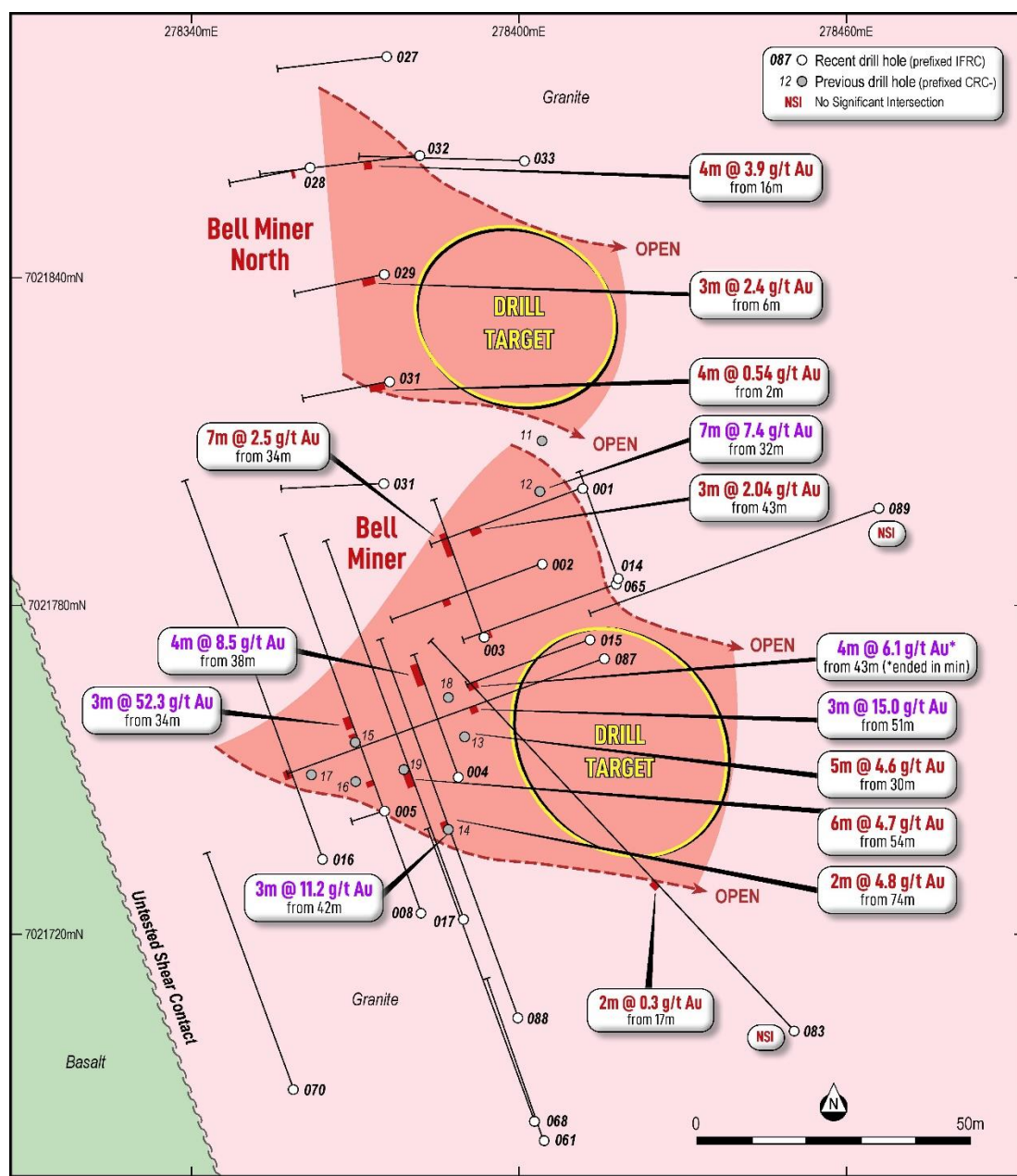
Figure 5: Interpreted geology map of the Ives Find granite intrusive showing the distribution of RC and diamond drill holes and significant drilling intersections
