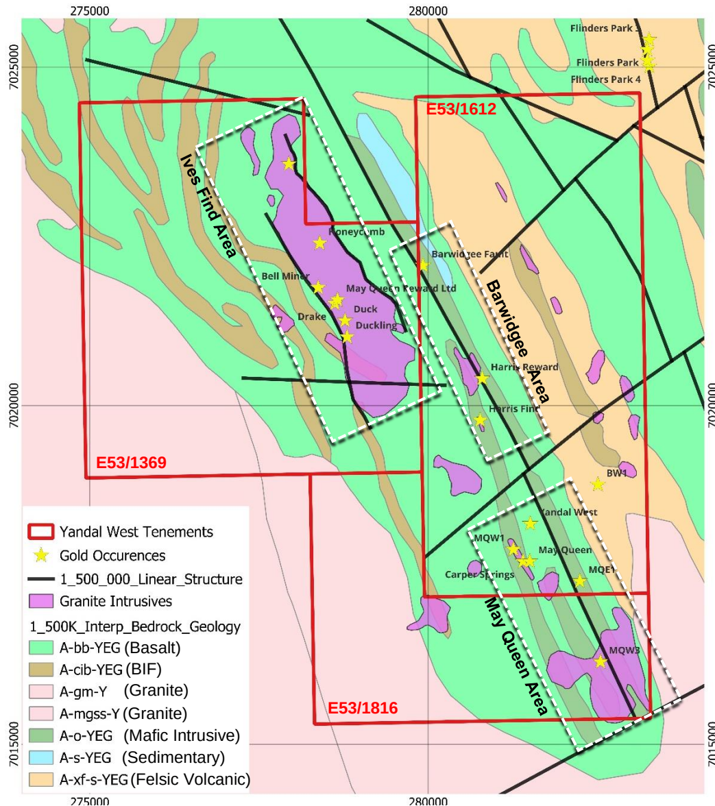
Figure 2: GSWA 1:500,000 bedrock geology map and the location of the granite and porphyry intrusives (from GSWA 1:250,000 surface geology map) and location of main gold occurrences.
