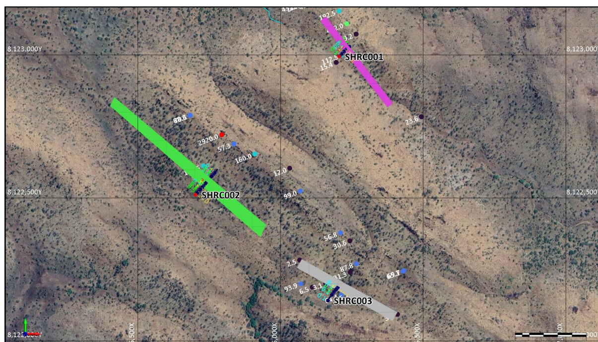
The best rock chip result likewise came from a gossanous outcrop on the hill located in front of SHRC002 and returned 0.29% Cu and 0.07% Co (Figure 8).
