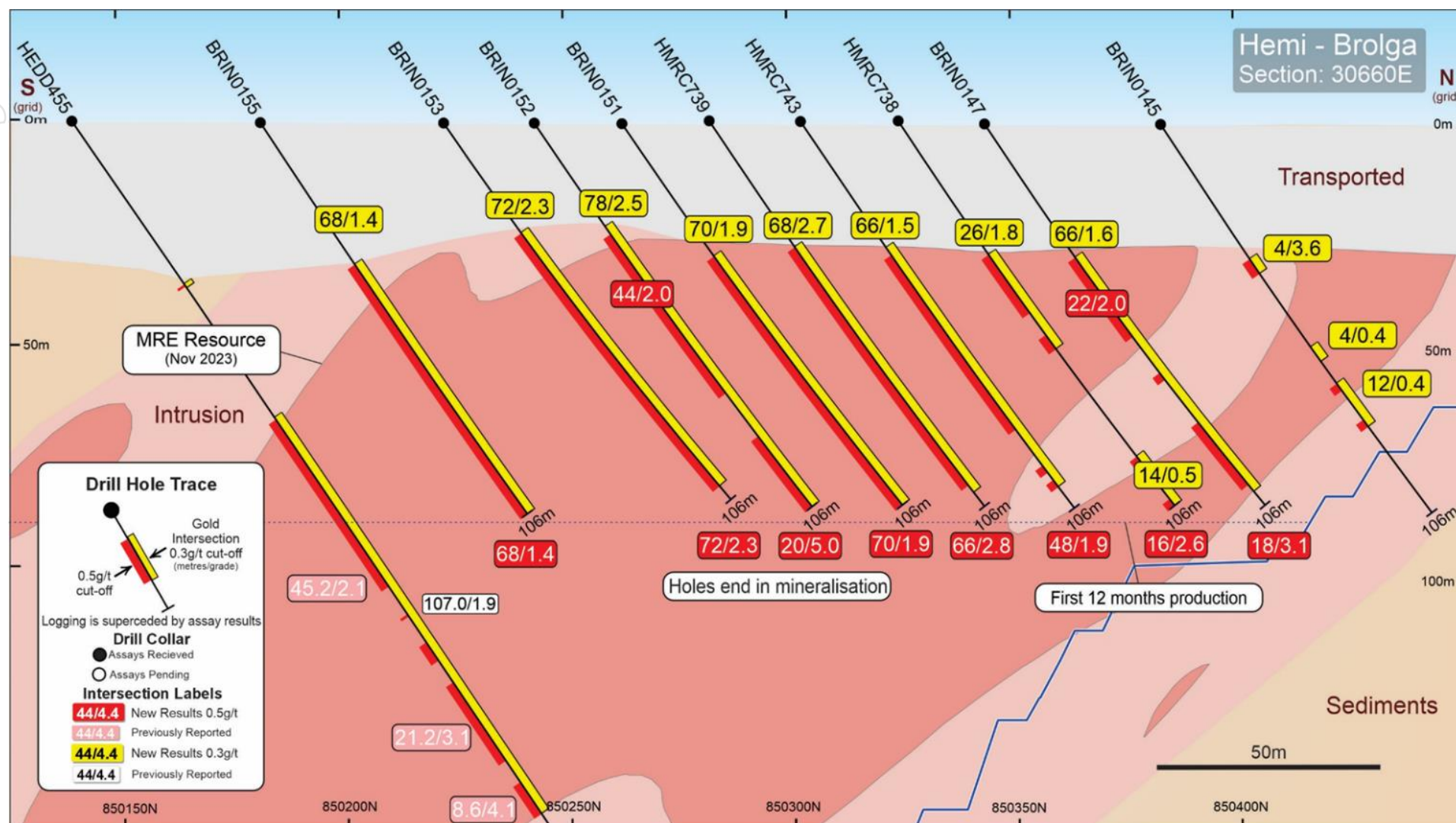
Figure 5 Brolga Cross Section 30660E
