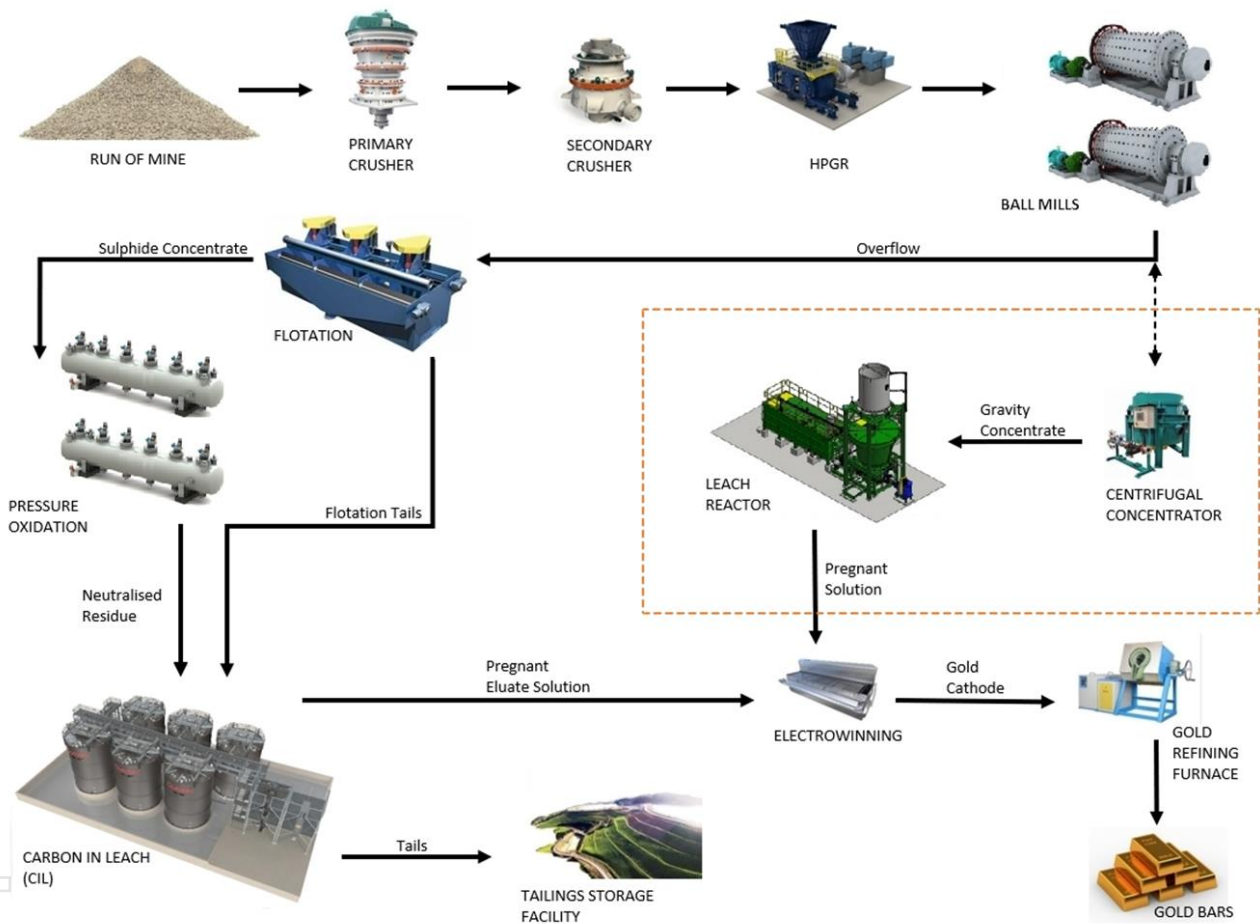
Figure 5 Metallurgical flowsheet.
