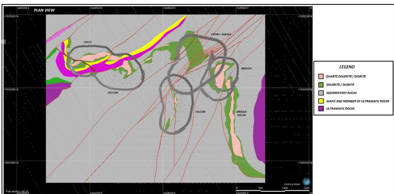
Figure 1 Plan flitch diagram of the geology and structures (red lines) at the Hemi Project.
