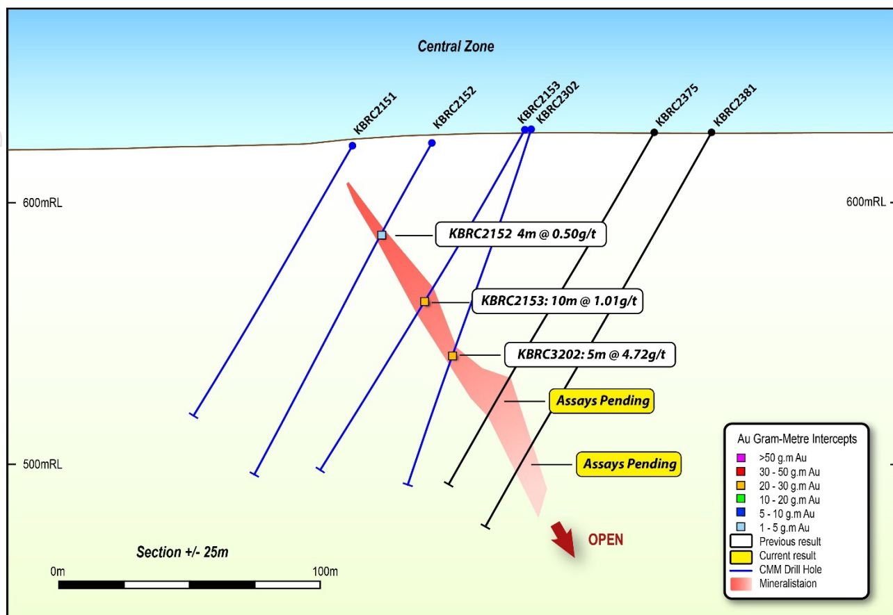
Figure 11: Central Lode cross-section 7366660mN with previous intercepts and inferred down dip extension of recent drilling observations. Refer to chip tray photos in Figures 12 & 13 below.
