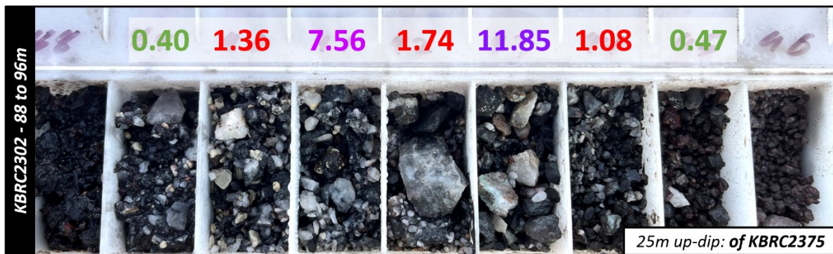
Figure 12: KBRC2302 chip tray 88 to 96m ore zone consisting of sulphidic shale (pyrite, chalcopyrite, malachite, molybdenite & sphalerite), brecciated quartz and carbonates, with Au ppm assay results top.
