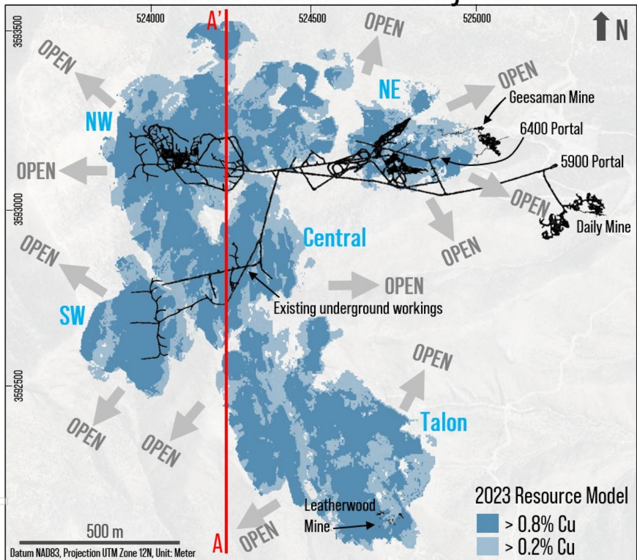
Figure 5 – Plan view of the new resource model at a 0.2% and 0.8% Cu cut-off grade, location of existing underground workings and main deposit areas.
