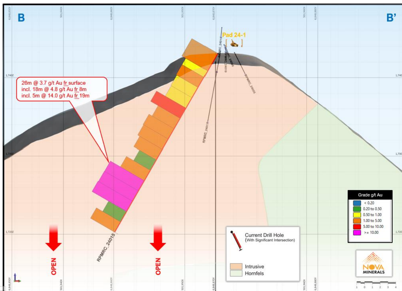
Figure 3. RPM North Section B-B' _220azi showing continuity of mineralization
